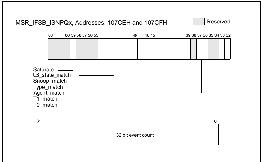
Figure 18-32. MSR_IFSB_ISNPQx, Addresses: 107CEH and 107CFH
