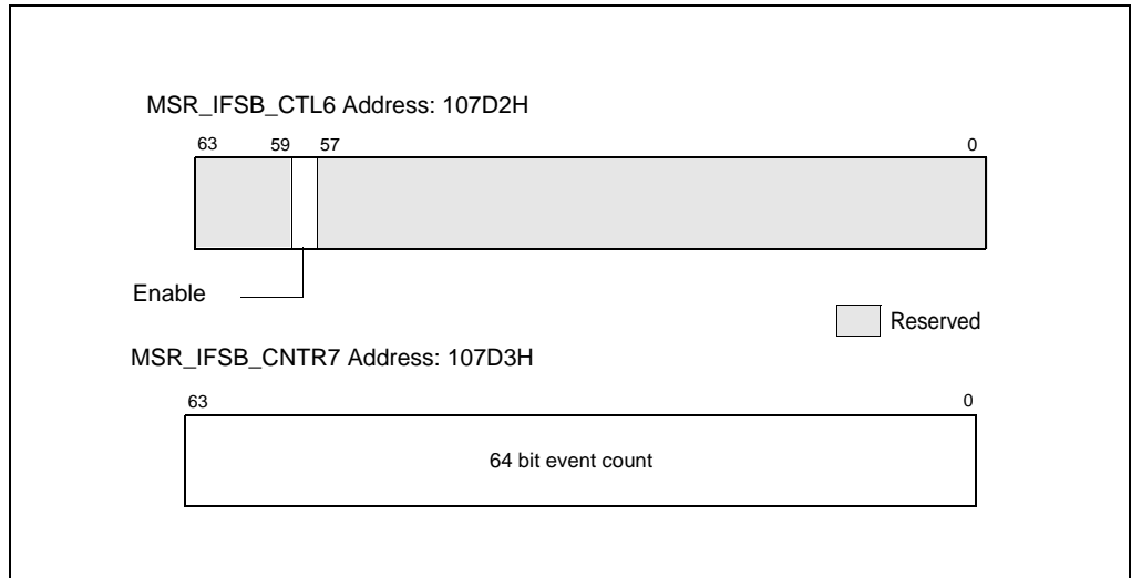
Figure 18-34. MSR_IFSB_CTRL6, Address: 107D2H; MSR_IFSB_CNTR7, Address: 107D3H
