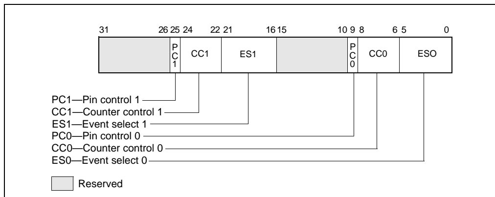
Figure 18-36. CESR MSR (Pentium Processor Only)
