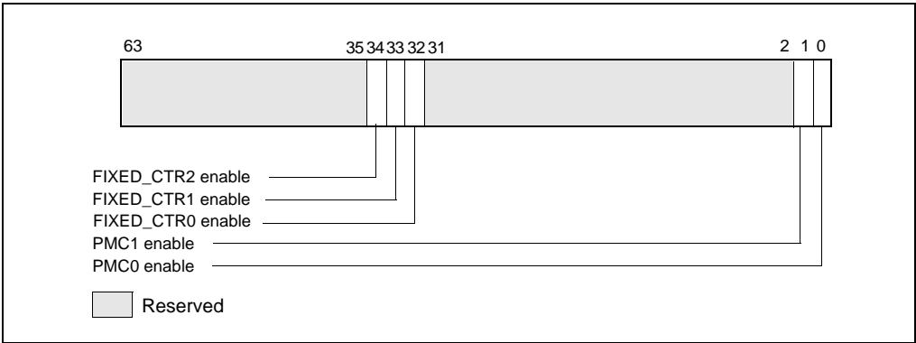
Figure 18-15. Layout of MSR_PERF_GLOBAL_CTRL MSR
