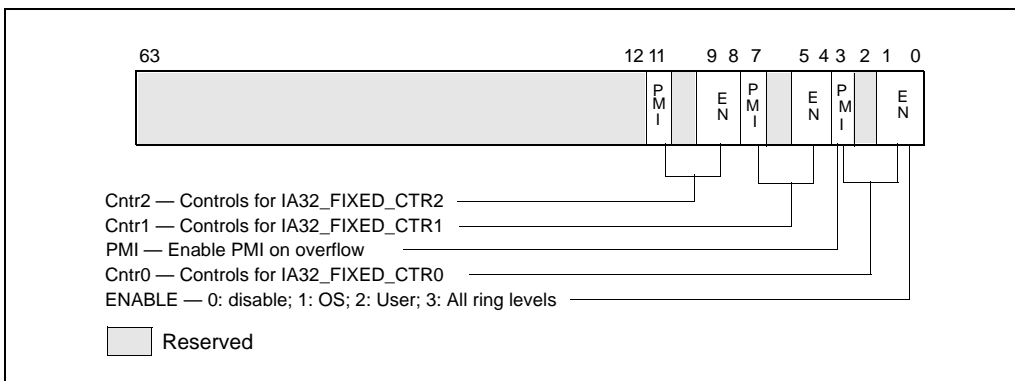
Figure 18-14. Layout of MSR_PERF_FIXED_CTR_CTRL MSR
