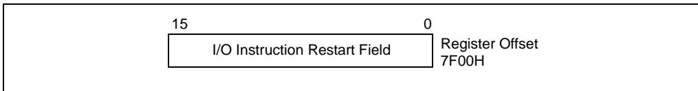
Figure 24-5. I/O Instruction Restart Field
