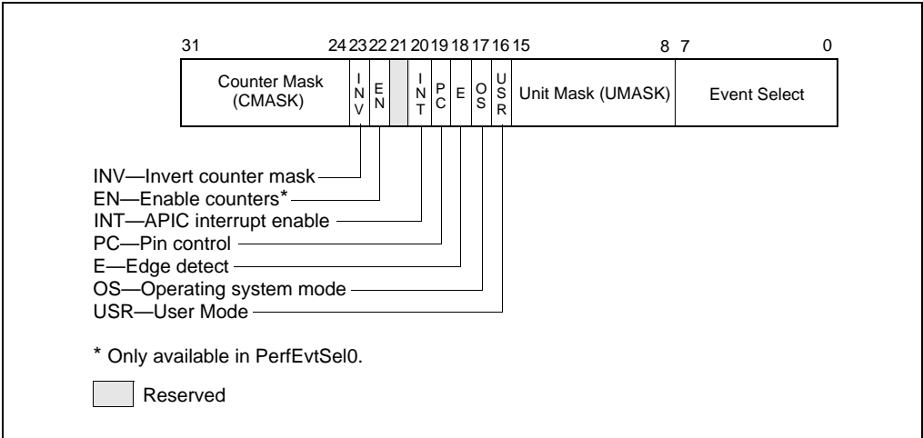
Figure 18-35. PerfEvtSel0 and PerfEvtSel1 MSRs
