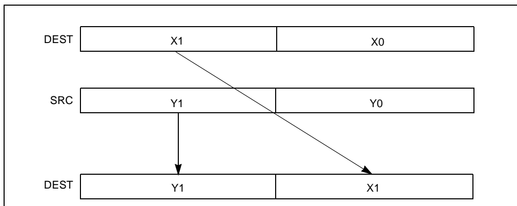
Figure 3-19. UNPCKHPD Instruction High Unpack and Interleave Operation
