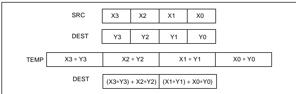
Figure 3-7. PMADDWD Execution Model Using 64-bit Operands
