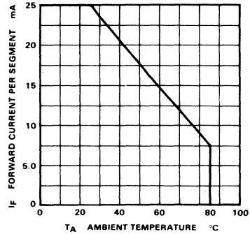
Maximum Average Current Rating vs Ambient Temperature
