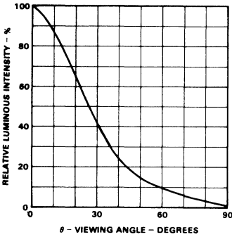
Angular Distribution of Luminous Intensity
