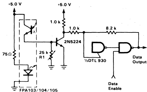
Interfacing Circuit
