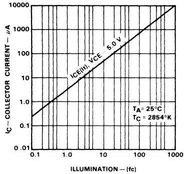
Photo Current Characteristics
