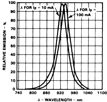
Emission Spectrum
