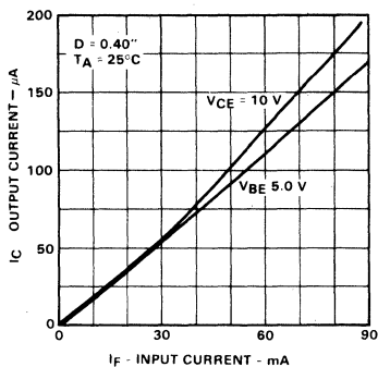
Output Current vs Input Current
