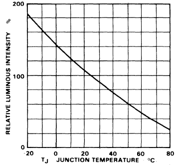
Relative Luminous Intensity vs Junction Temperature
