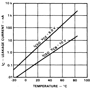
Collector Dark Current vs Temperature
