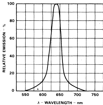
Emission Spectrum
