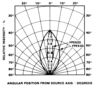
Radiation Pattern
