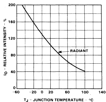
Intensity vs Temperature
