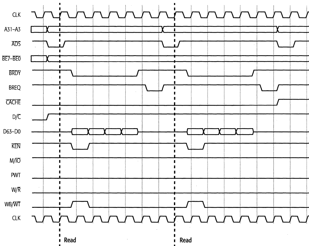
FIGURE 5-6. Burst Reads
