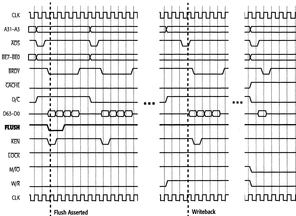
FIGURE 5-22. FLUSH-Acknowledge Cycle
