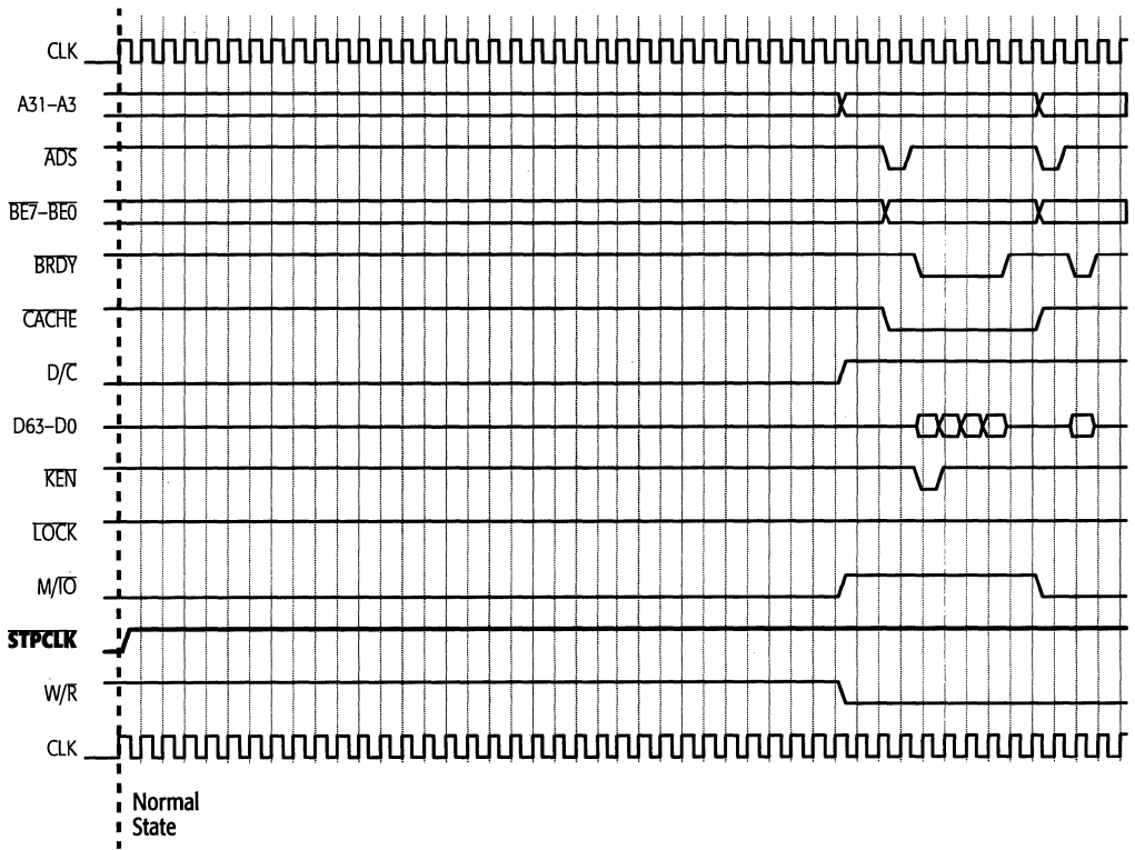
FIGURE 5-27B. Stop-Grant and Stop-Clock Modes Part 2
