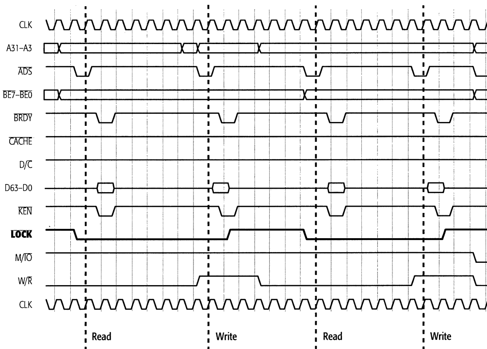
FIGURE 5-16. Basic Locked Operation
