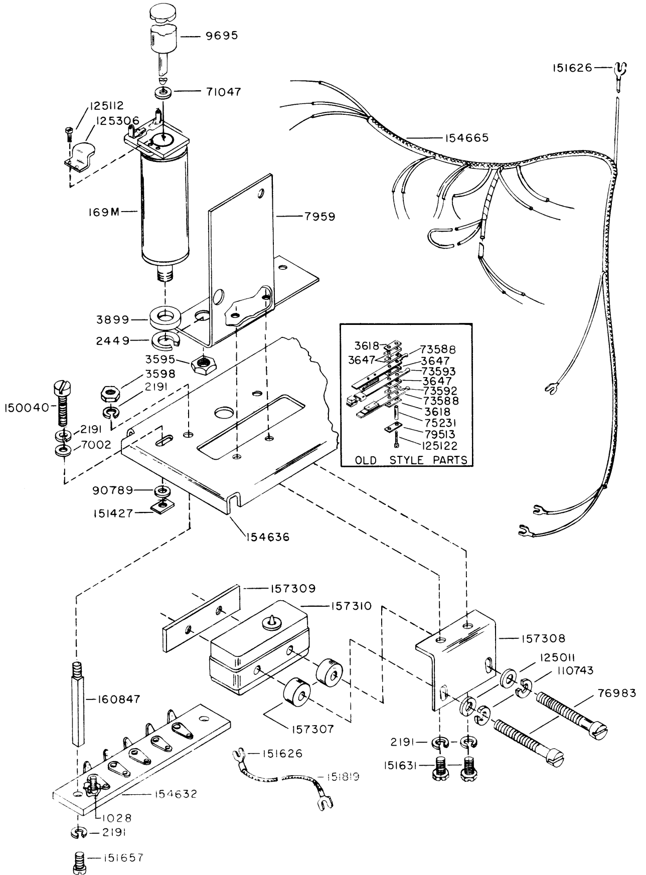
FIGURE 6-13. 152332 RELAY MOTOR CONTROL ASSEMBLY
