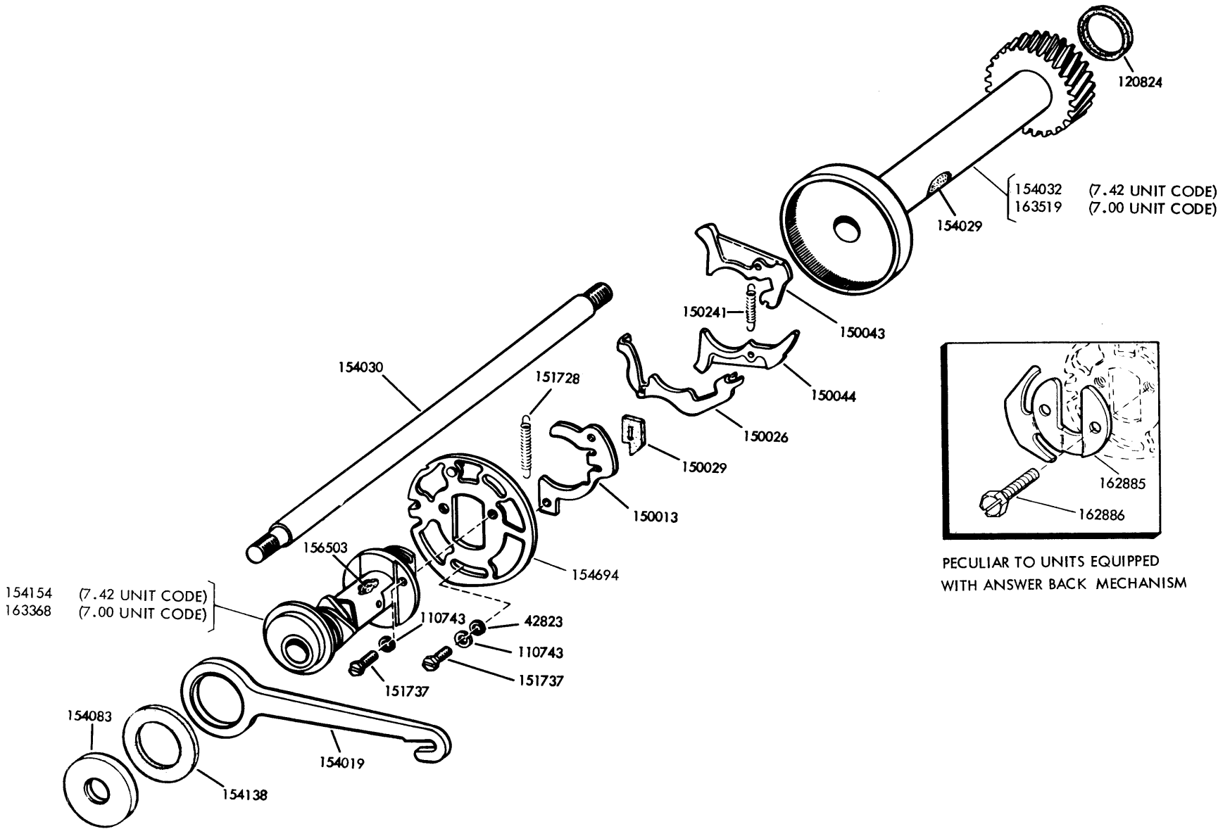
FIGURE 2-10. SIGNAL GENERATOR SHAFT MECHANISM
