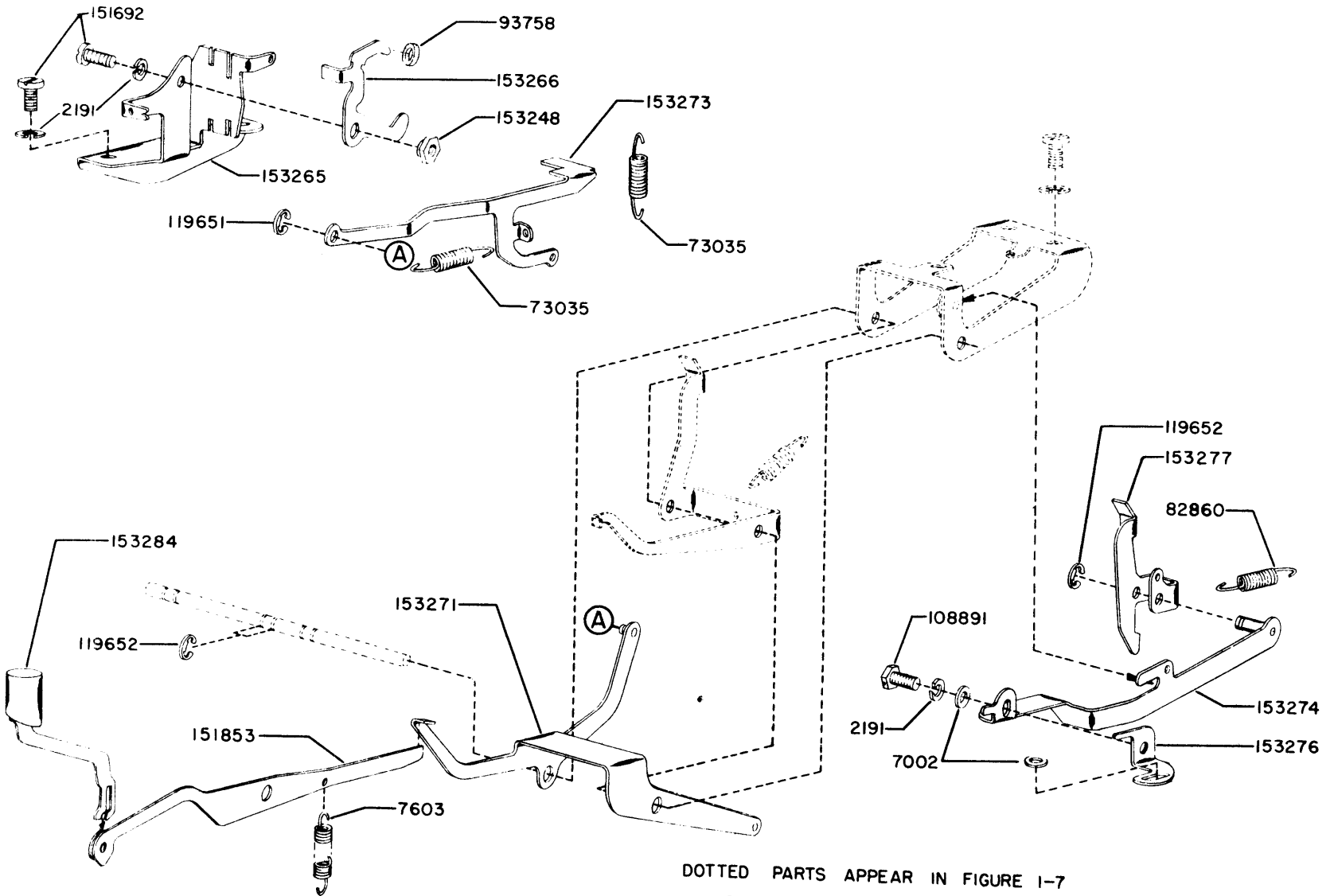
FIGURE 1-24. 152918 MODIFICATION KIT TO PROVIDE LOCAL BACK SPACE MECHANISM (MARK II KEYBOARD)
