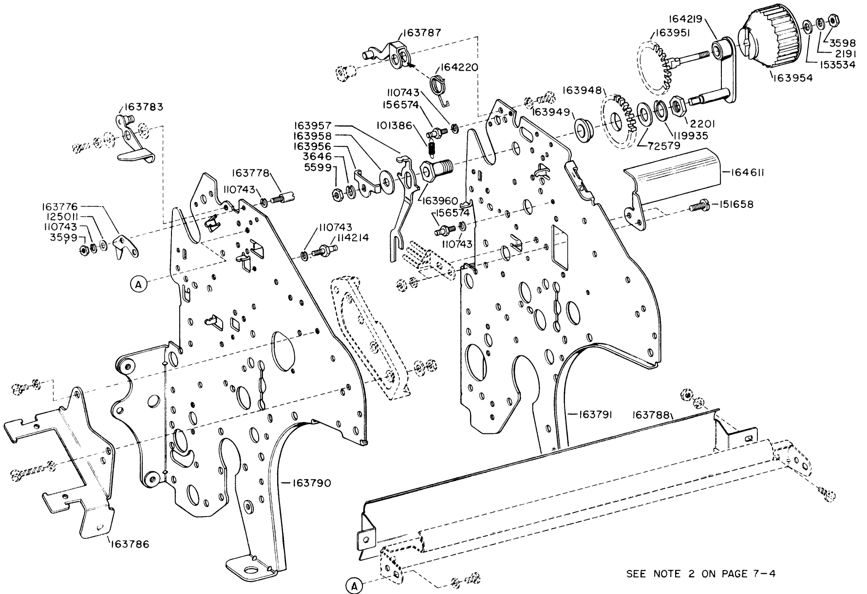
FIGURE 3-4 LEFT AND RIGHT SIDE FRAMES MECHANISM
