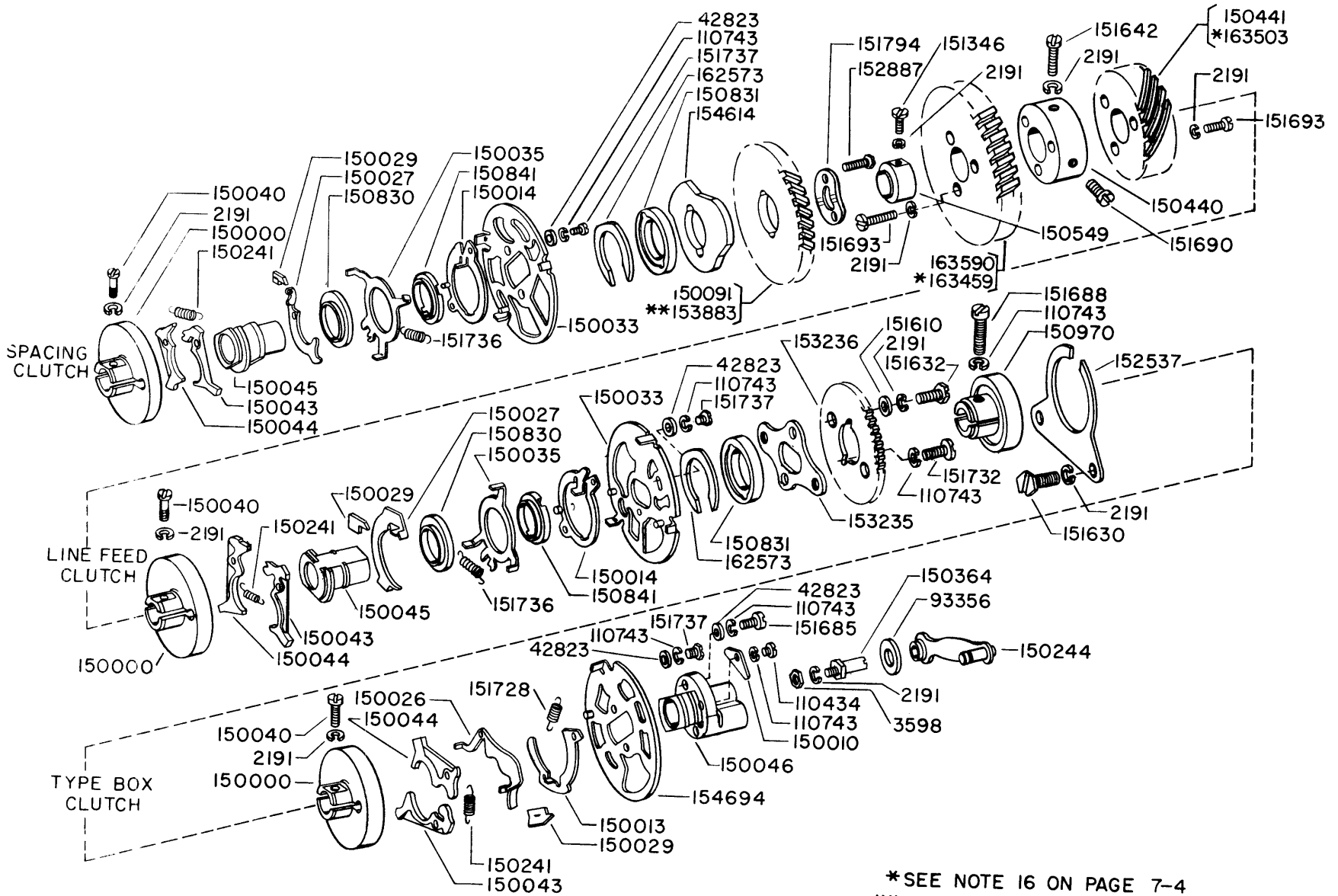
FIGURE 3-18. MAIN SHAFT MECHANISM
