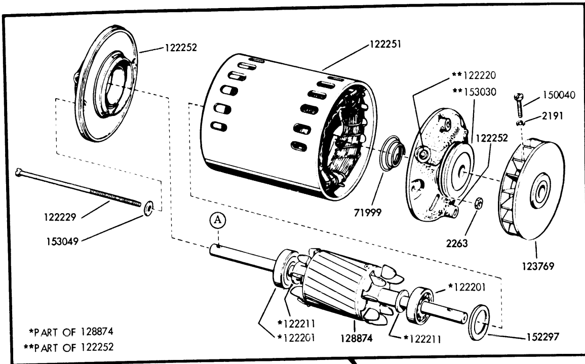
151795 (1/20 H. P., 115V/1/60 Cycle, A.C. Synchronous Motor (G.E. Model 5SC19LG3)
