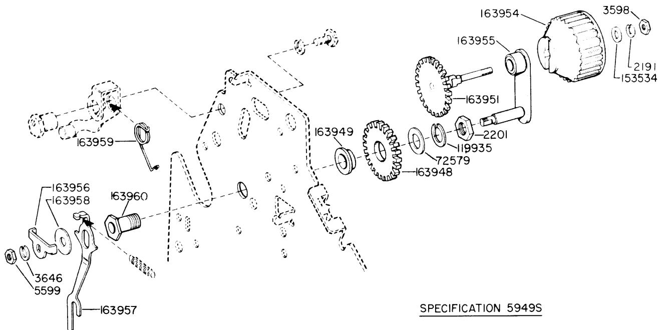
FIGURE 3-93. 163947 MODIFICATION KIT TO PROVIDE IMPROVED MANUAL PLATEN LINE FEED
