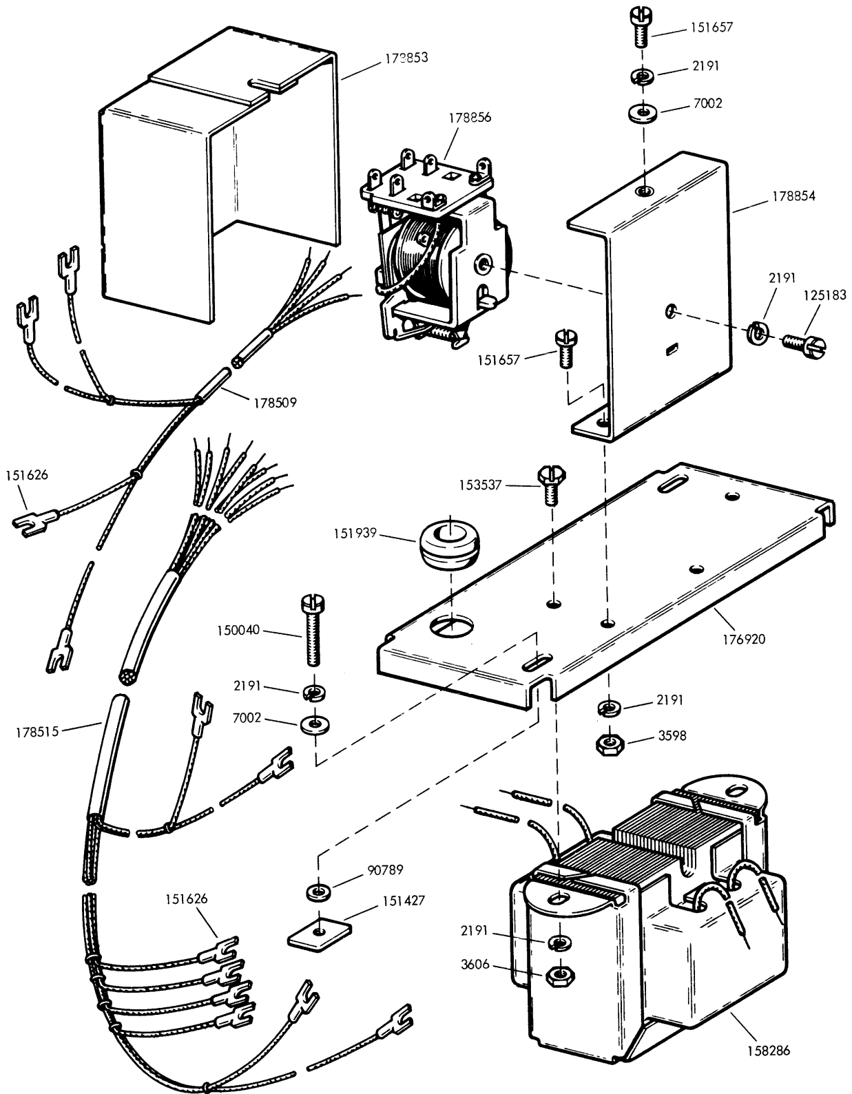
FIGURE 7A-10. 176921 TRANSFORMER AND RELAY ASSEMBLY
