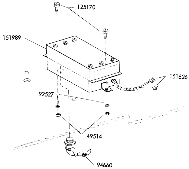
FIGURE 5-25. 151988 MODIFICATION KIT TO ADD POWER LINE ELECTRICAL NOISE SUPPRESSOR
