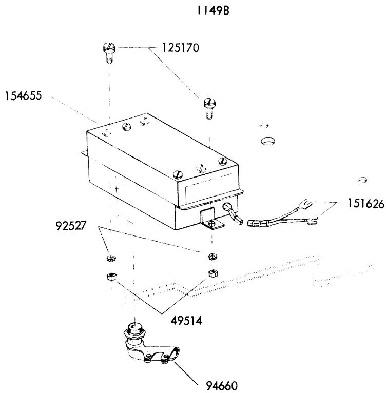
FIGURE 5-24. 154651 MODIFICATION KIT TO ADD SIGNAL LINE ELECTRICAL NOISE SUPPRESSOR (D.C.)
