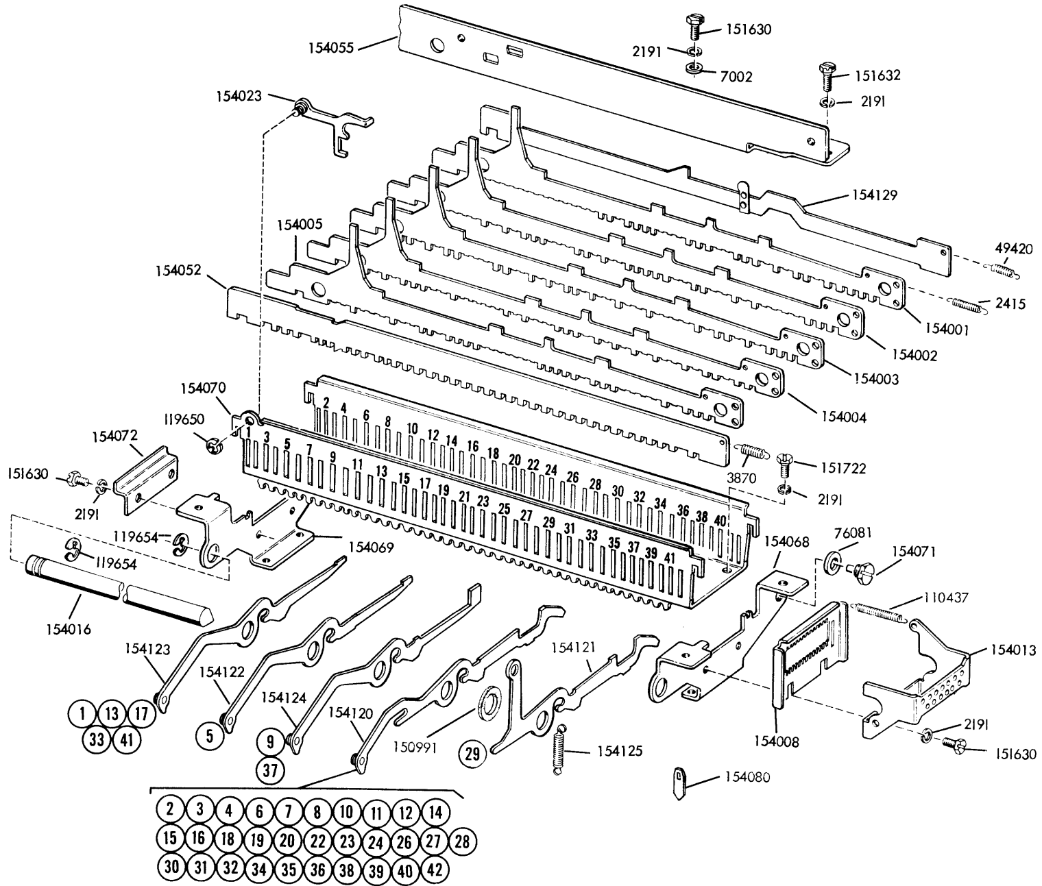
FIGURE 2-6. CODE BAR MECHANISM
