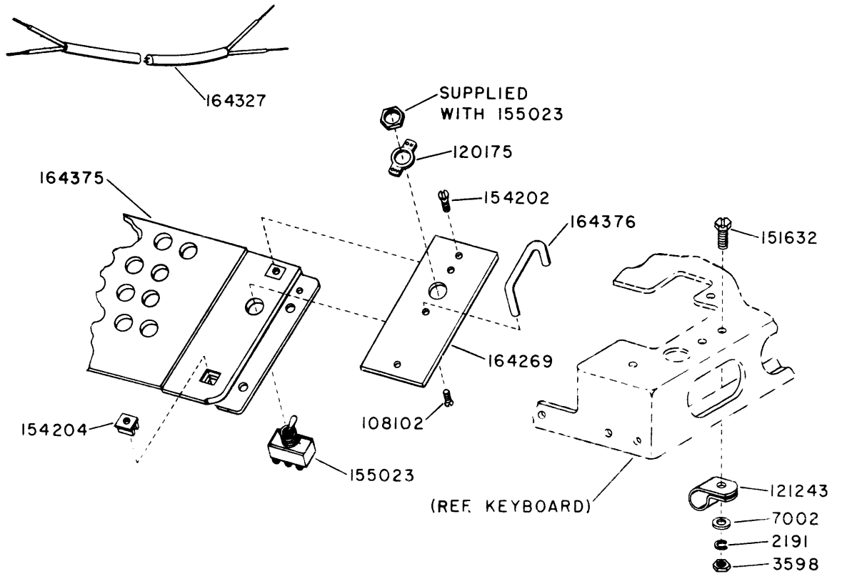
FIGURE 2-5. VARIABLE FEATURES OF KEYBOARD MECHANISM
