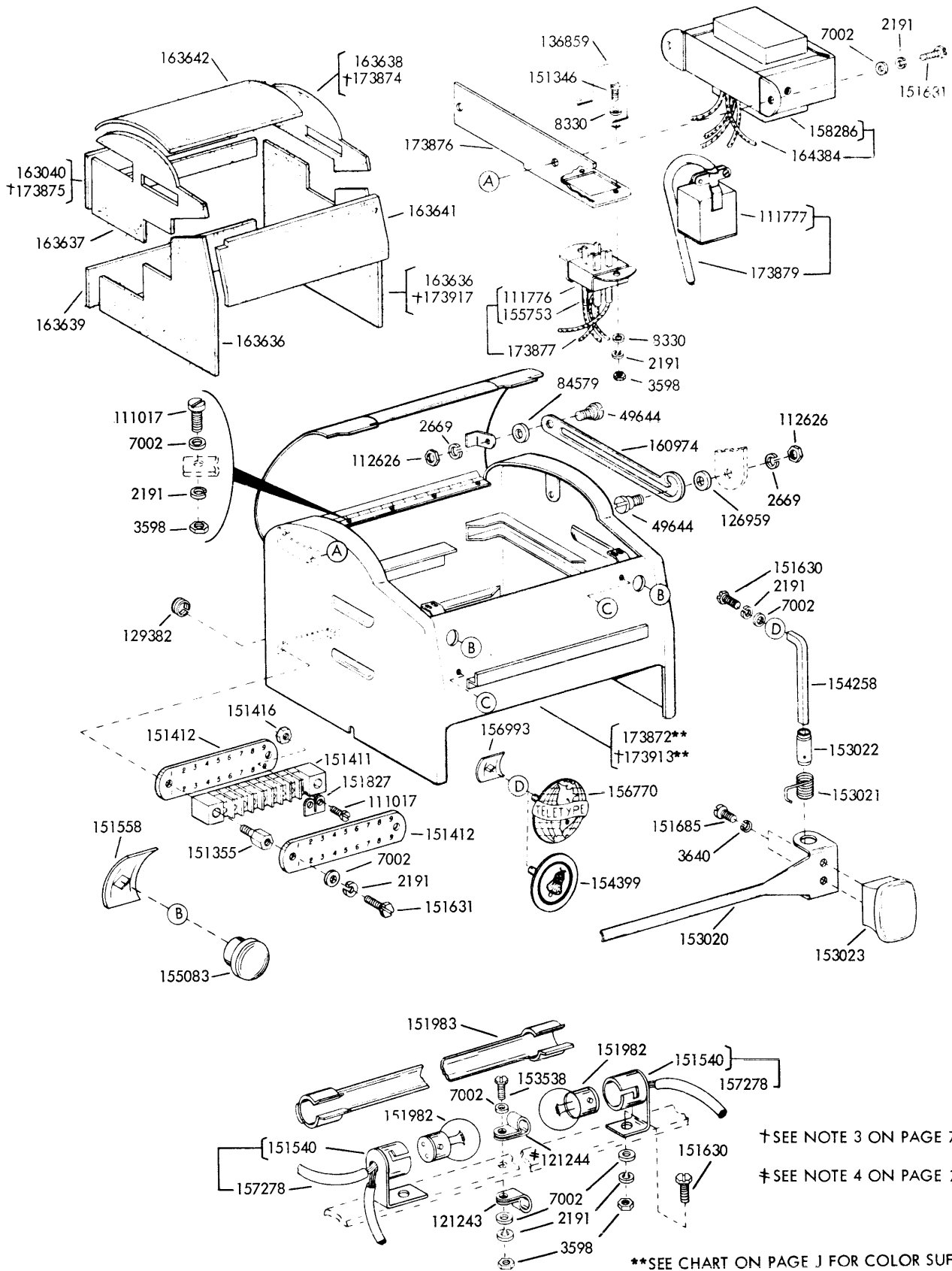
FIGURE 5-34. LPC206** AND LPC207** COVERS
