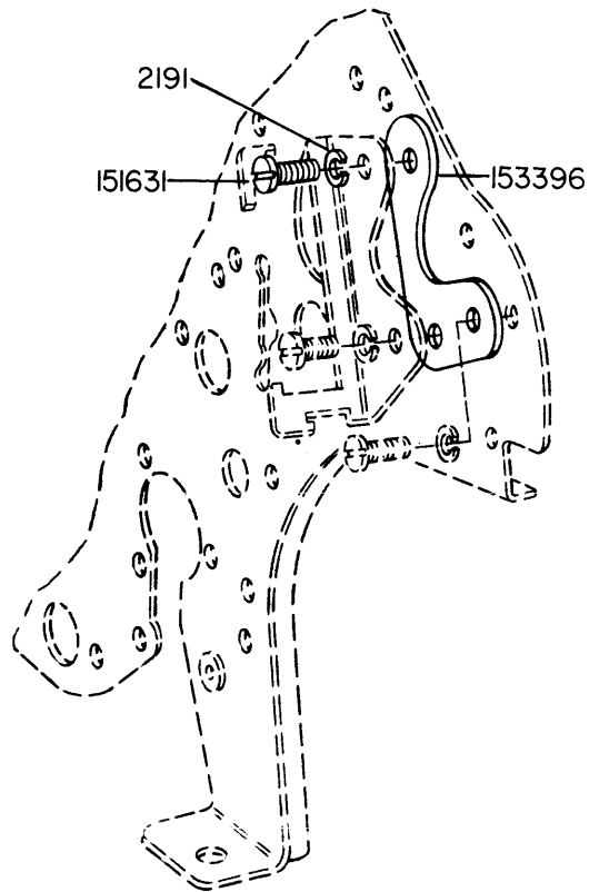
FIGURE 3-58. 153912 MODIFICATION KIT TO PROVIDE FIGS.—LTRS. CODE BAR MANUAL SHIFTING
