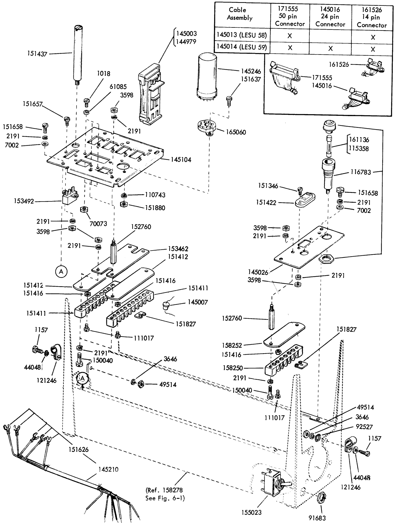
FIGURE 6-32. ELECTRICAL SERVICE UNIT
