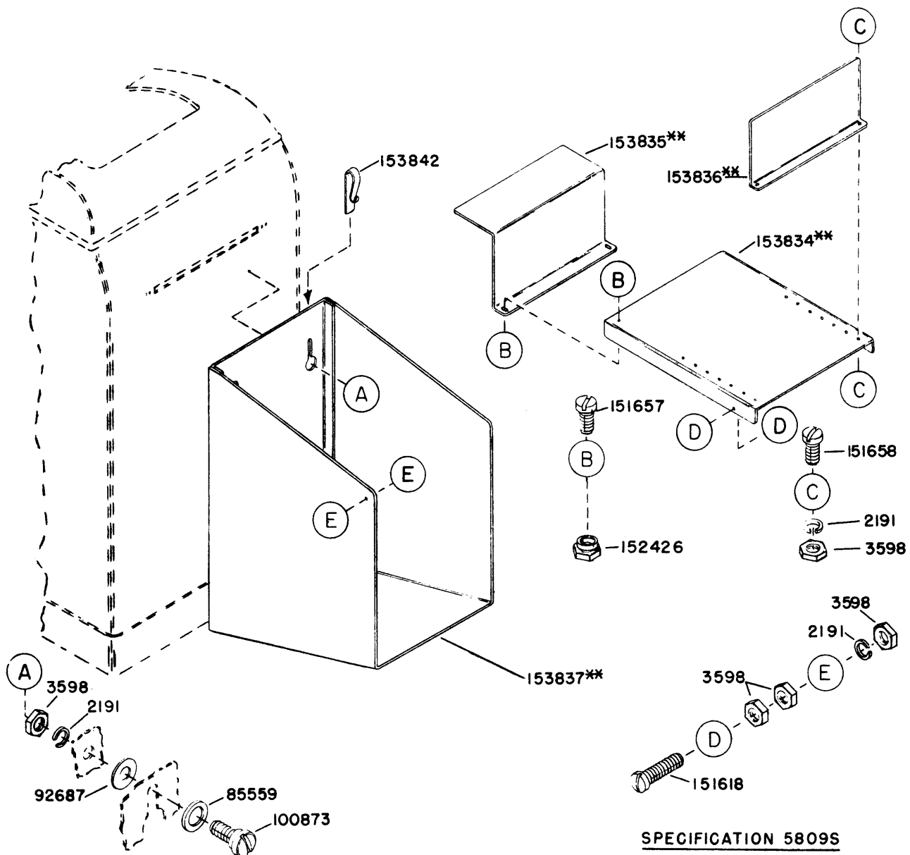
FIGURE 5-4. 152349** MODIFICATION KIT TO PROVIDE PAPER SUPPLY AND ACCUMULATING SHELF
