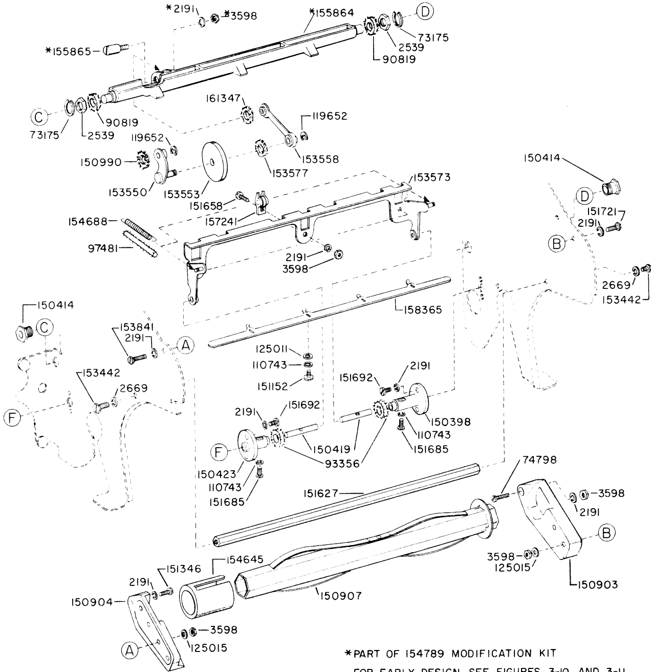
FIGURE 3-9. PAPER SPINDLE AND RESET BAIL MECHANISM
