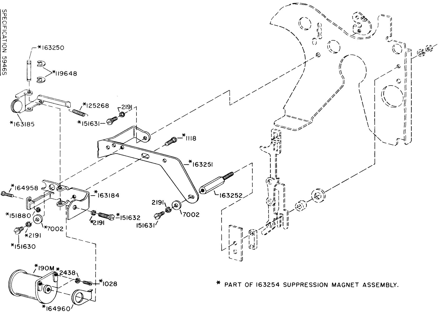
FIGURE 3-92. 163183 MODIFICATION KIT TO PROVIDE D.C. MAGNET OPERATED PRINT SUPPRESSION
