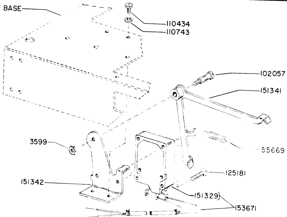
FIGURE I-19. 152343 MODIFICATION KIT TO PROVIDE END-OF-LINE SWITCH MECHANISM
