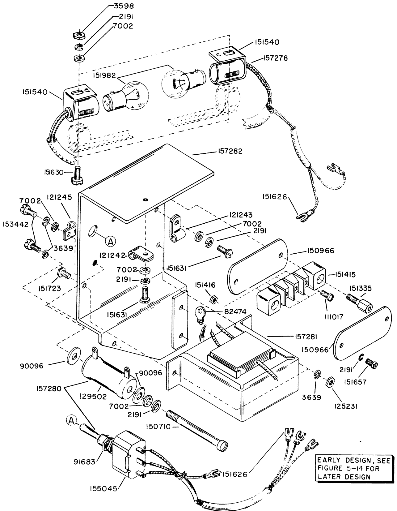
FIGURE 5-15. 6 VOLT A. C. INCANDESCENT COPYLIGHT SYSTEM
