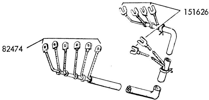
FIGURE 6-17. 160223 AUXILIARY CABLE ASSEMBLY
