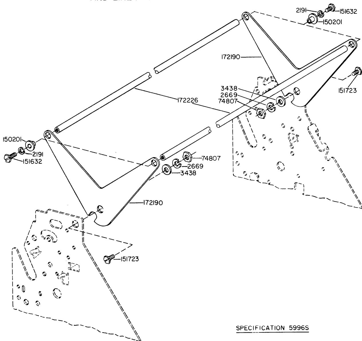
FIGURE 3-96. 157514 MODIFICATION KIT TO PROVIDE AUTOMATIC CARRIAGE RETURN AND LINE FEED
