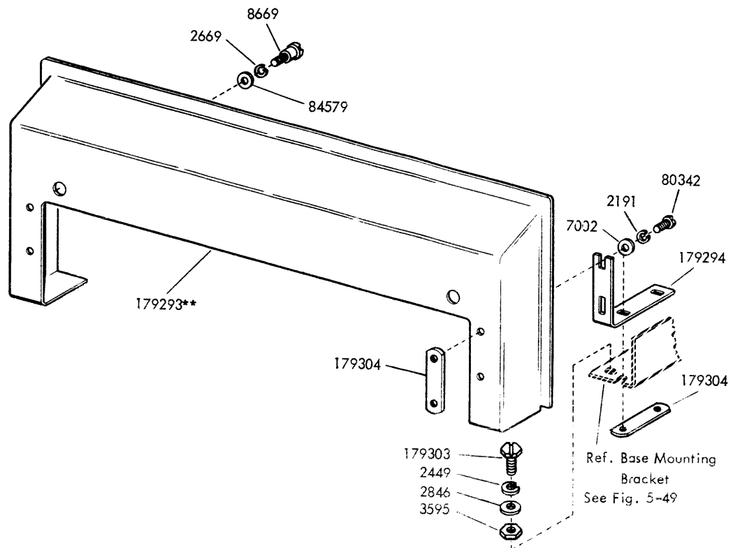
FIGURE 5-65. KEYBOARD PANEL ASSEMBLY (LBAC233**)
