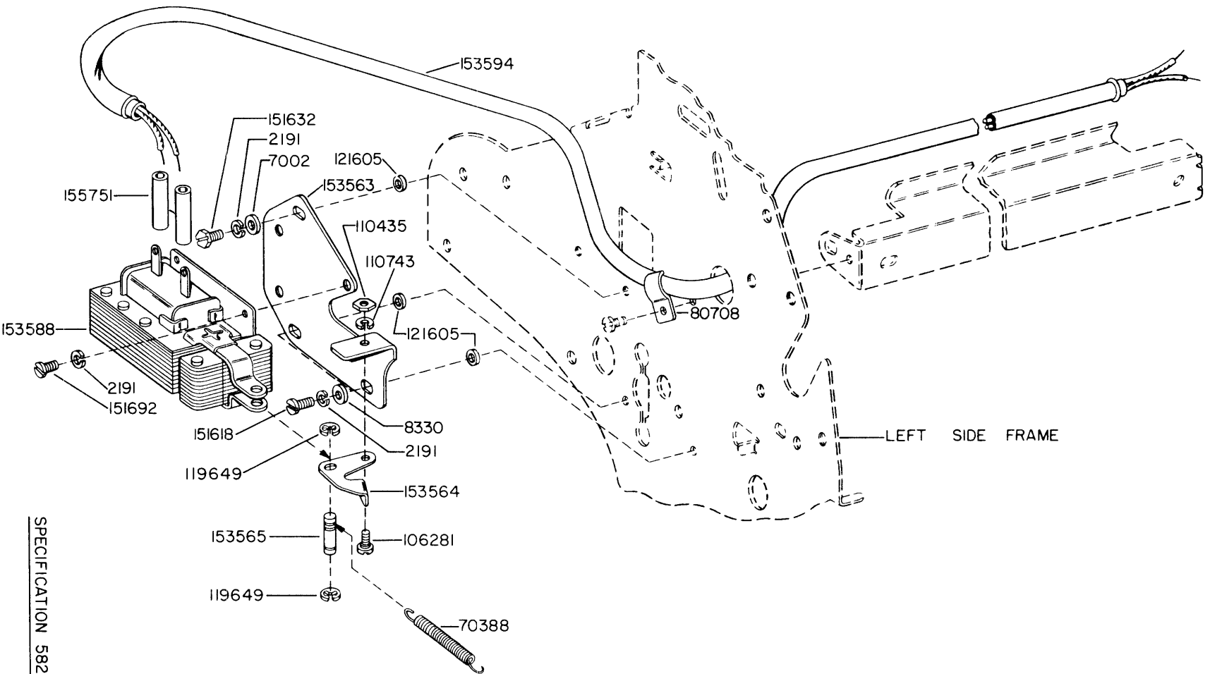
FIGURE 3-64. 152345 MODIFICATION KIT TO PROVIDE OFF-LINE STUNT SHIFT CONTROL
