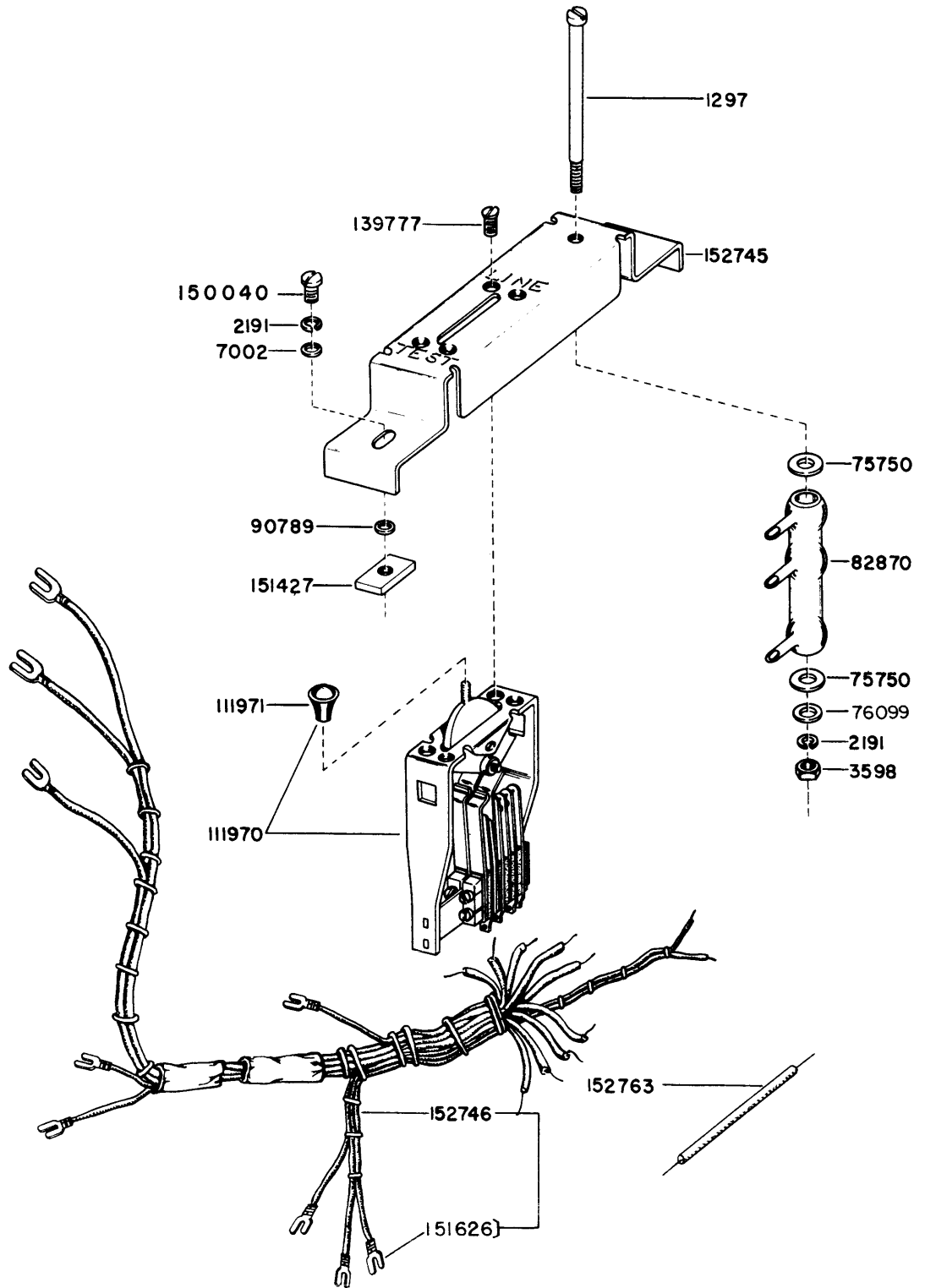
FIGURE 6-9. 152744 LINE TEST KEY ASSEMBLY
