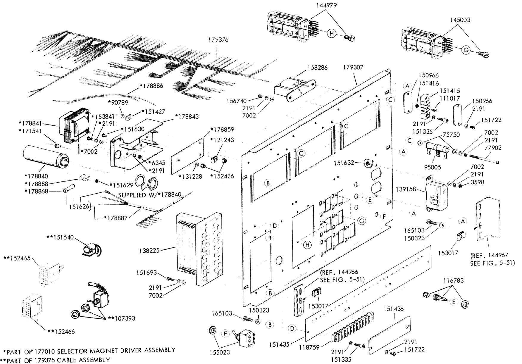
FIGURE 5-69. ELECTRICAL SERVICE ASSEMBLY (LBAC233**)
