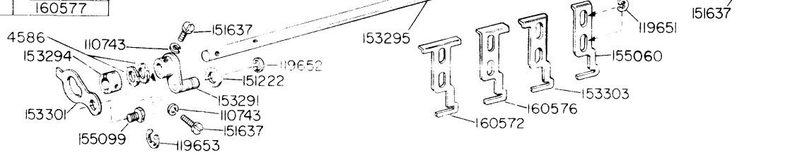
FIGURE 3-44 STUNT BOX-MAJOR COMPONENT VARIABLES
