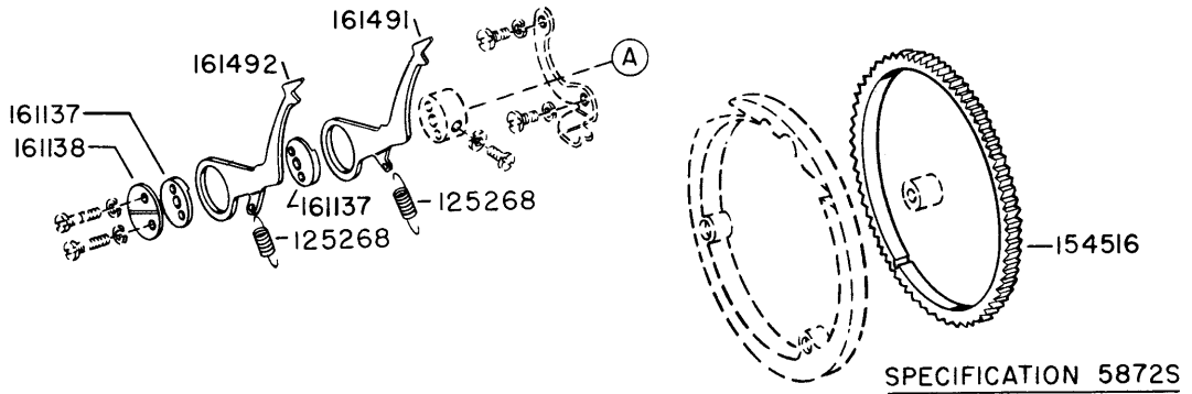
FIGURE 3-78. 159395 MODIFICATION KIT TO PROVIDE 6 SPACES PER INCH HORIZONTALLY
