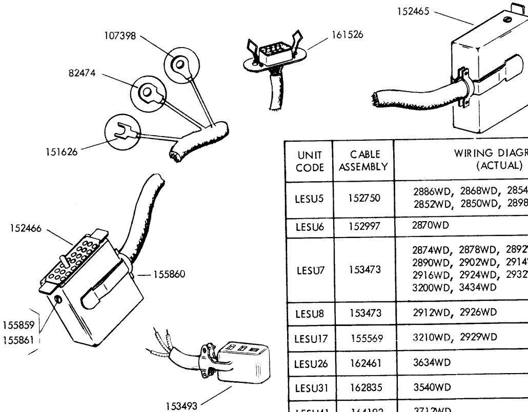
FIGURE 6-23. VARIABLE FEATURES FOR ELECTRICAL SERVICE UNIT
