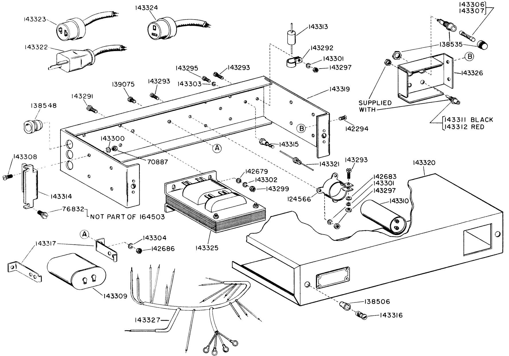
FIGURE 6-27. I64503 RECTIFIER ASSEMBLY
