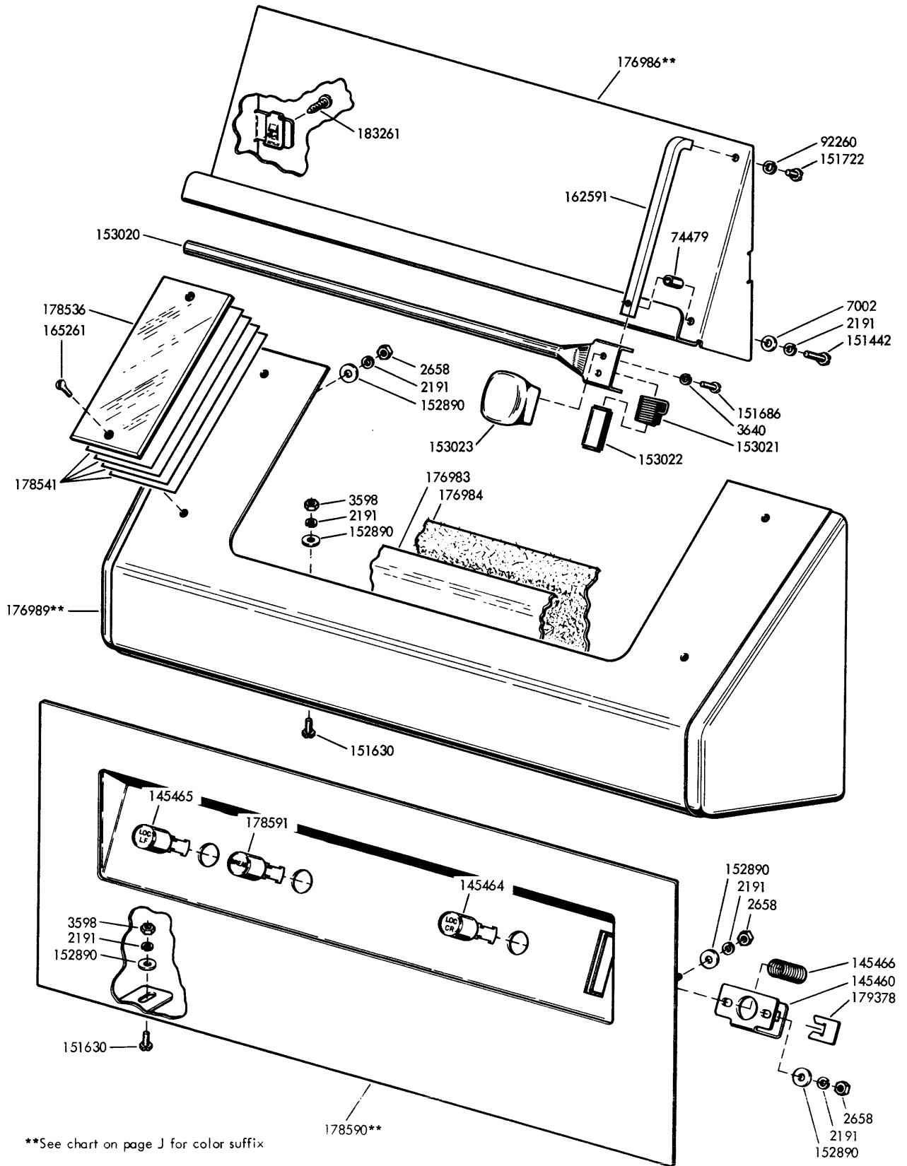
FIGURE 7A-17. COPYHOLDER TRAY, HOOD AND FRONT PLATE
