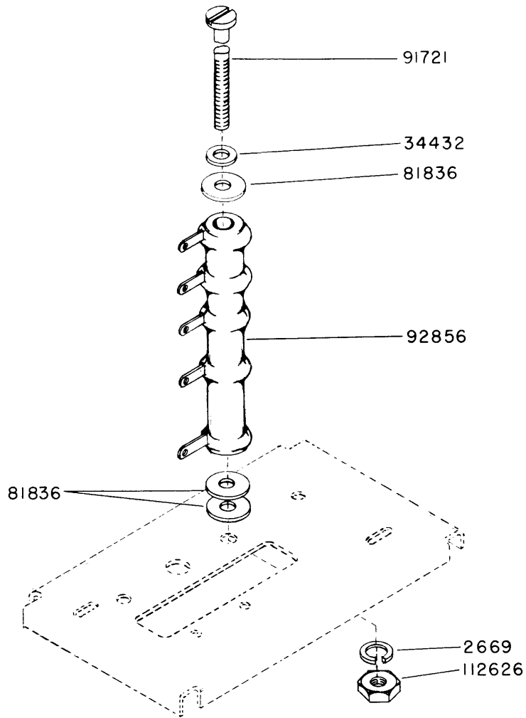
FIGURE 6-14. 93073 1500 OHM RESISTOR MODIFICATION KIT
