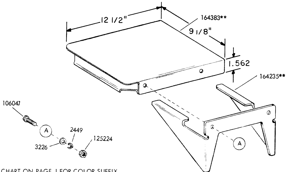
FIGURE 5-27. 163796**MODIFICATION KIT TO PROVIDE SHELF FOR CONSOLE CABINET
