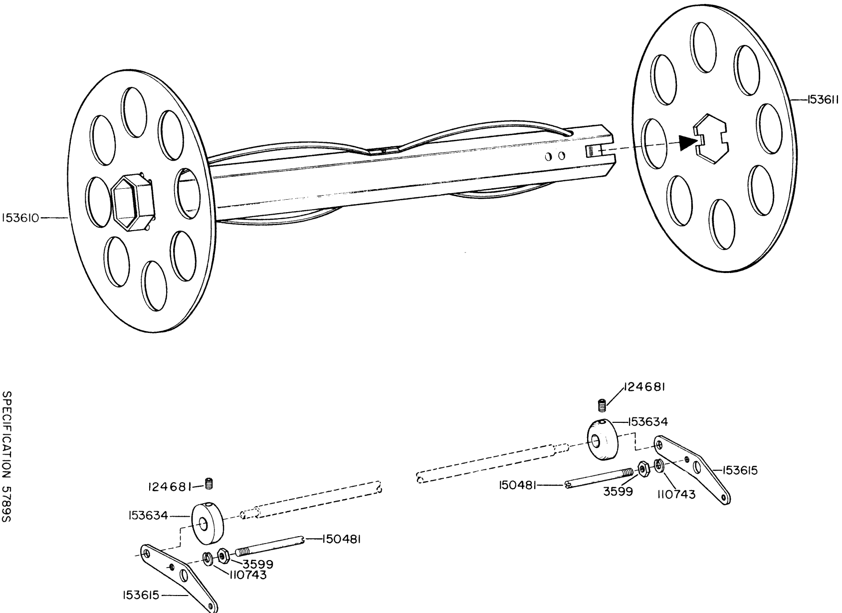
FIGURE 3-63 152340 MODIFICATION KIT TO PROVIDE MULTI-COPY PAPER HANDLING
