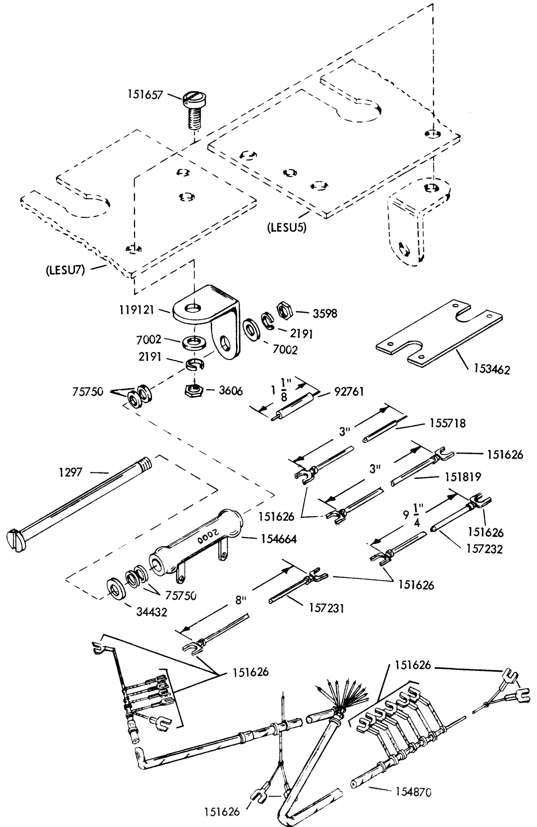
FIGURE 6-19. 154747 MODIFICATION KIT TO EQUIP AN ELECTRICAL SERVICE UNIT FOR CONTINUOUS SPACING
