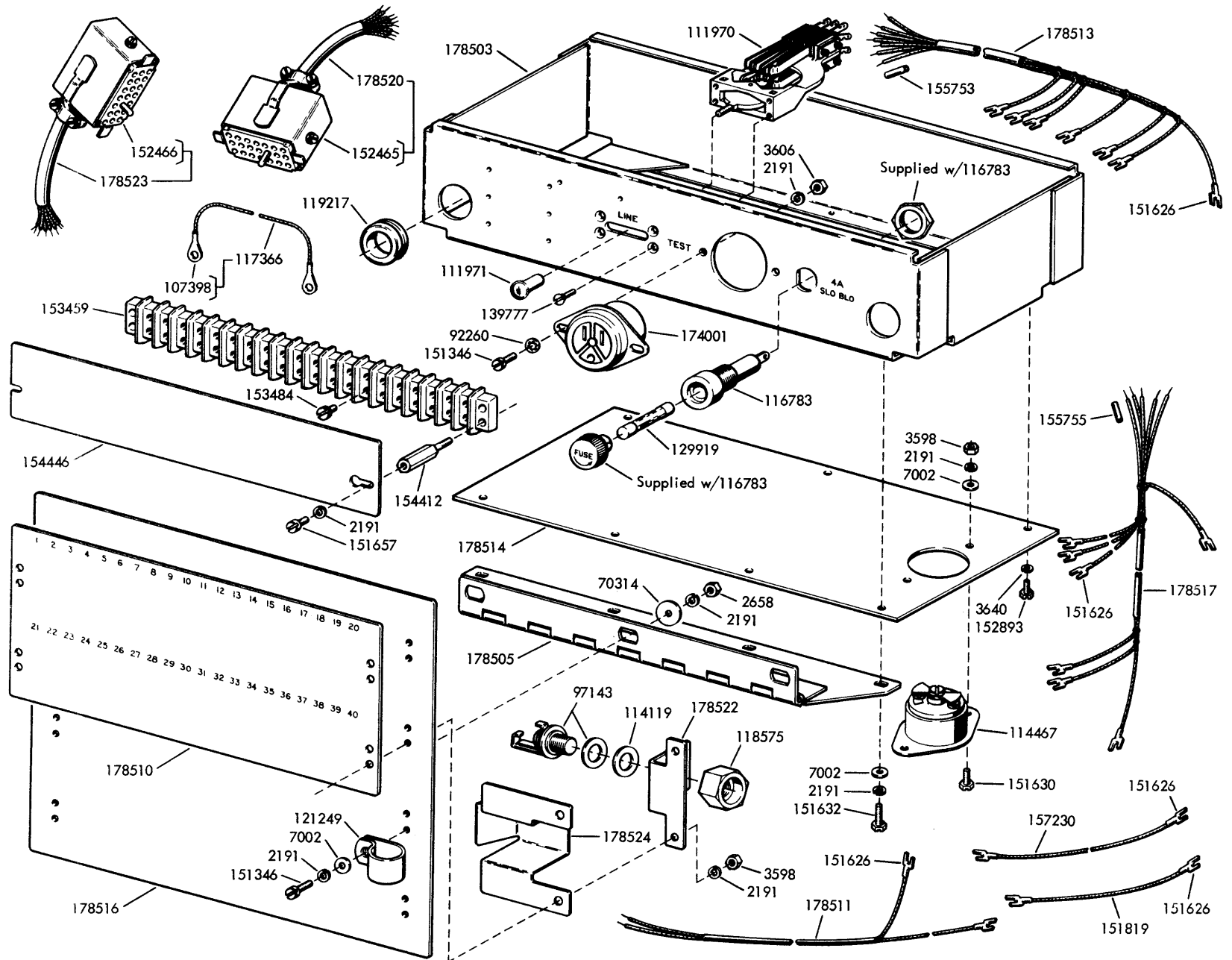
FIGURE 7A-9. ELECTRICAL SERVICE UNIT
