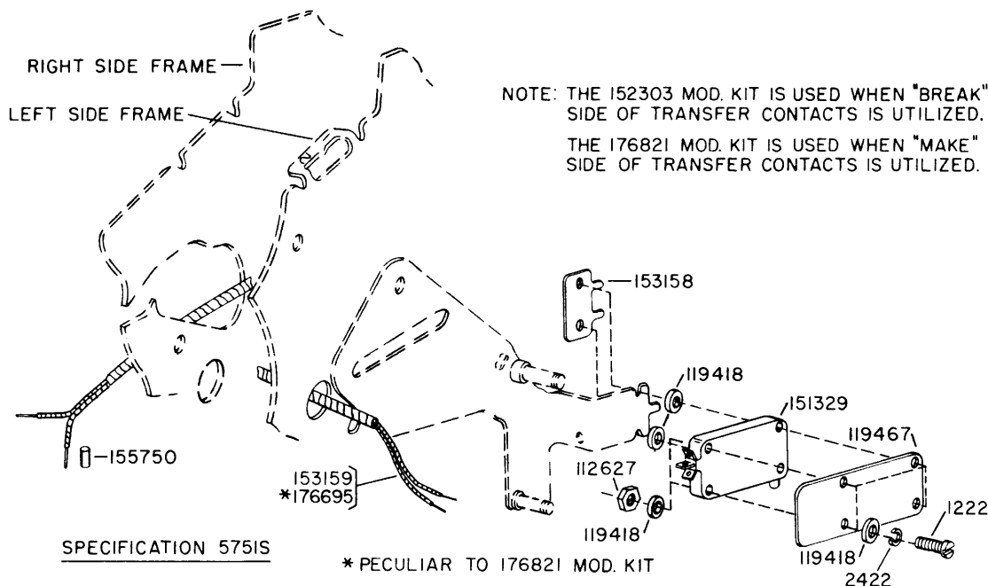
FIGURE 3-54. 152303 AND 176821 MODIFICATION KITS TO PROVIDE PAGE FEED-OUT TRANSMITTER CONTROL
