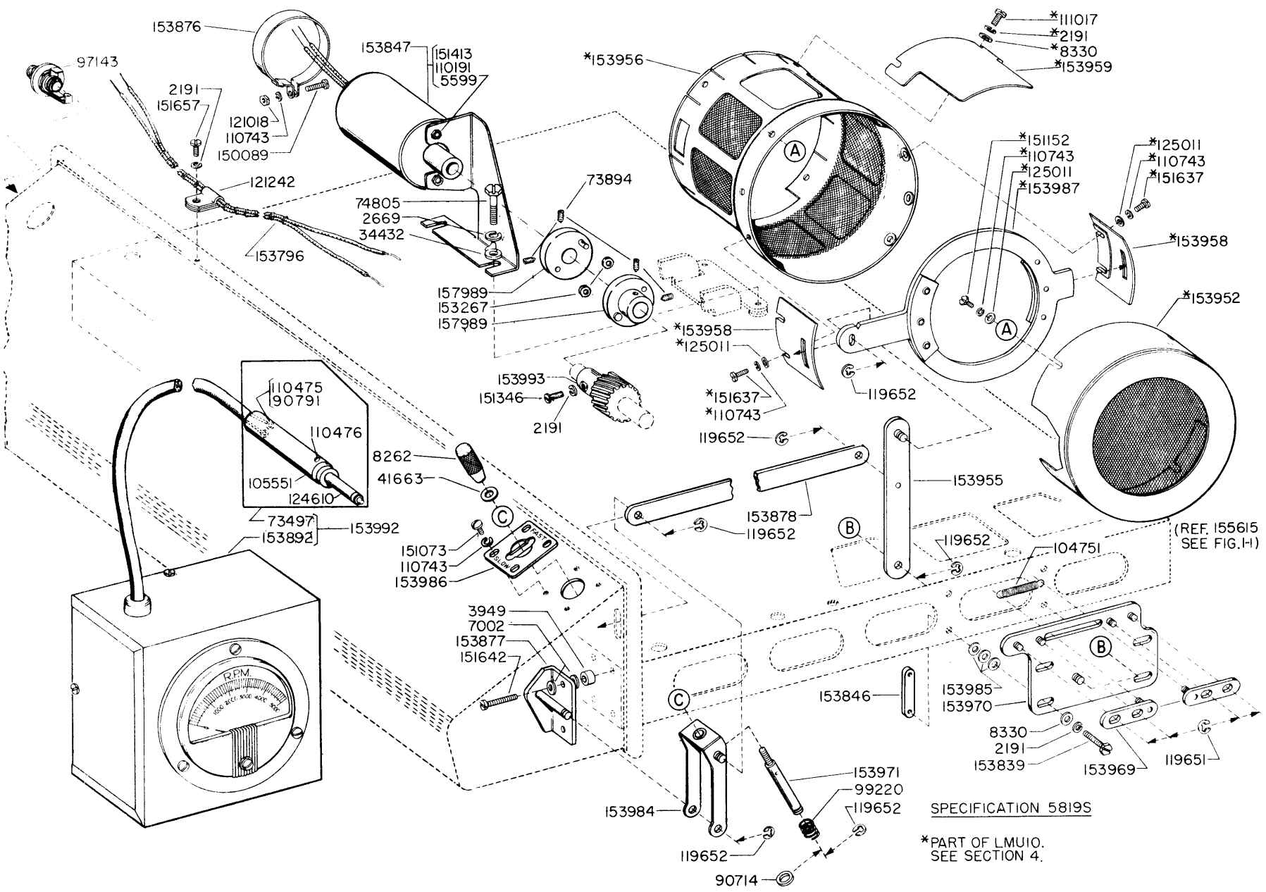
FIGURE 1-30. TACHOMETER AND GOVERNOR ADJUSTMENT LINKAGE
