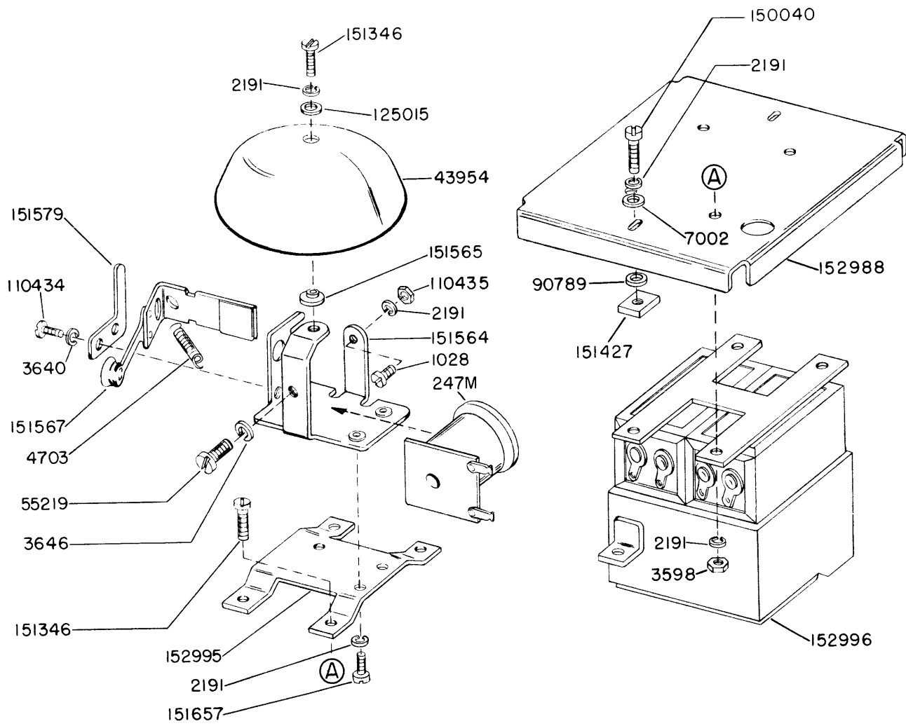
FIGURE 6-31. 152999 FILTER AND BELL ASSEMBLY
