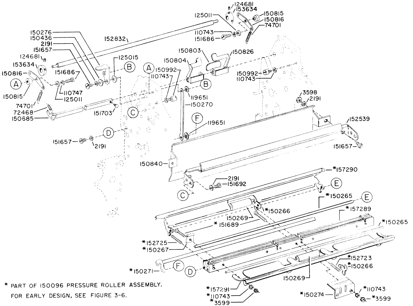
FIGURE 3-5. PRESSURE ROLLER MECHANISM
