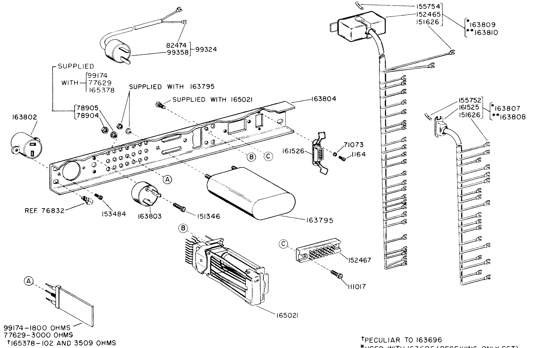
FIGURE 6-26. 163696 AND 163697 RELAY PANEL ASSEMBLIES
