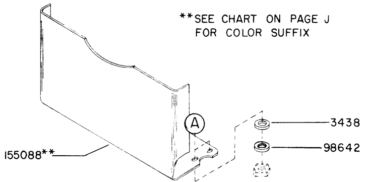
FIGURE 5-7. 152300** MODIFICATION KIT TO PROVIDE DIRECTORY HOLDER
