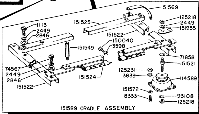
FIGURE 5-3. VARIABLE FEATURES FOR LAC203**, LAC204**, LAÇ213**, LAC215**, LAC216** CABINETS
