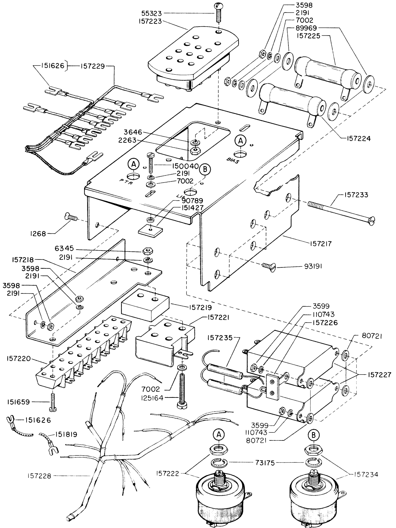
FIGURE 6-16. 157216 LINE RELAY MOUNTING ASSEMBLY
