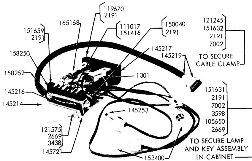
MODIFICATION KIT TO PROVIDE KEY AND LAMP ASSEMBLY
