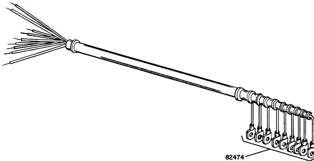
FIGURE 6-20. 155785 CABLE EXTENSION
