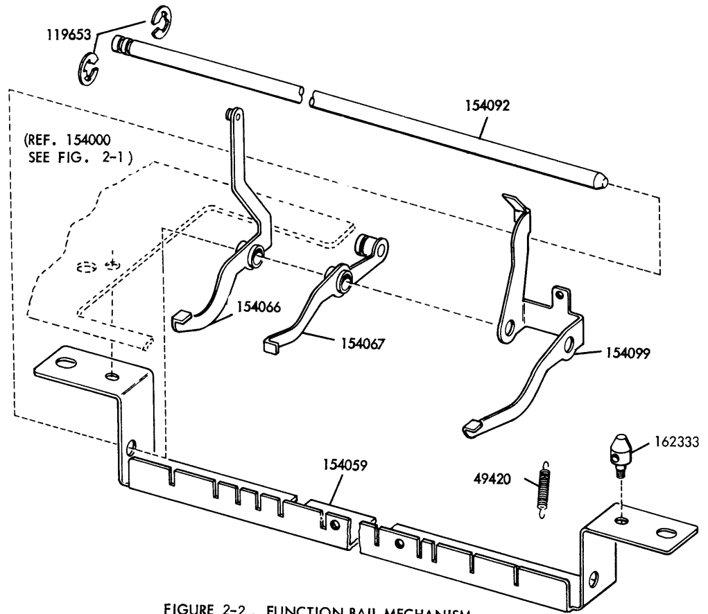
FIGURE 2-2 . FUNCTION BAIL MECHANISM
