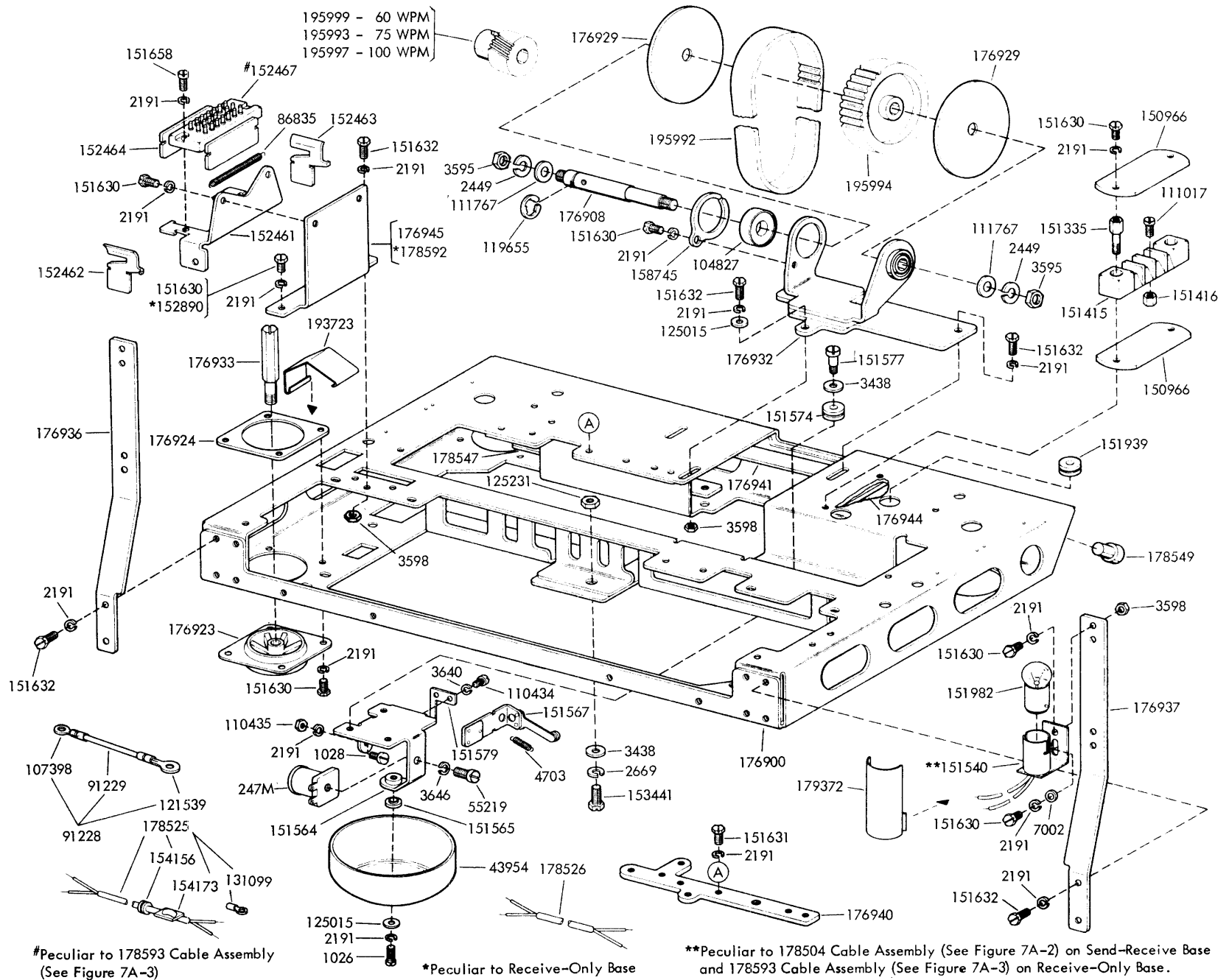
FIGURE 7A-1. KEYBOARD AND BASE MECHANISM
