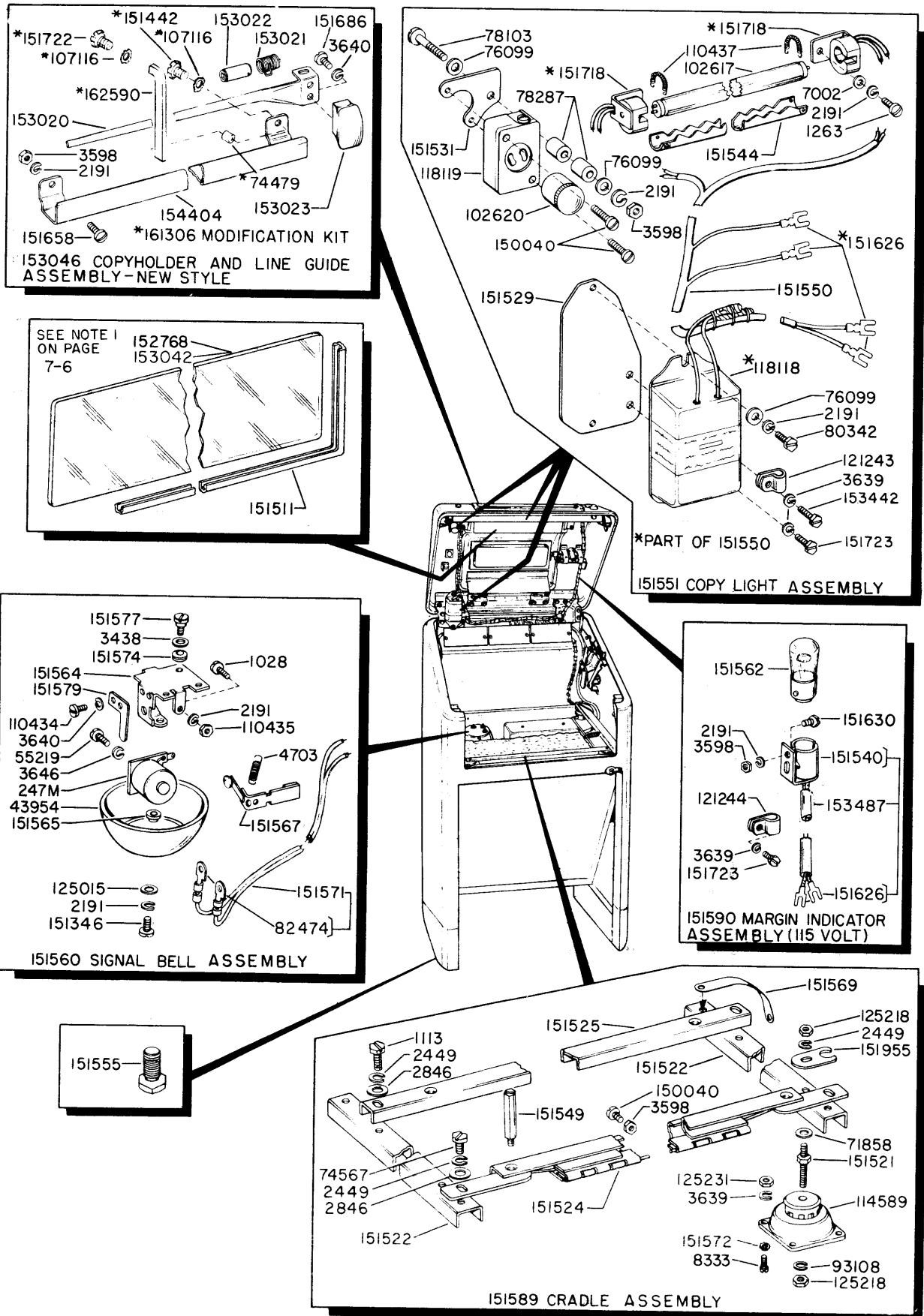
FIGURE 5-2. VARIABLE FEATURES FOR LAC202** CABINET
