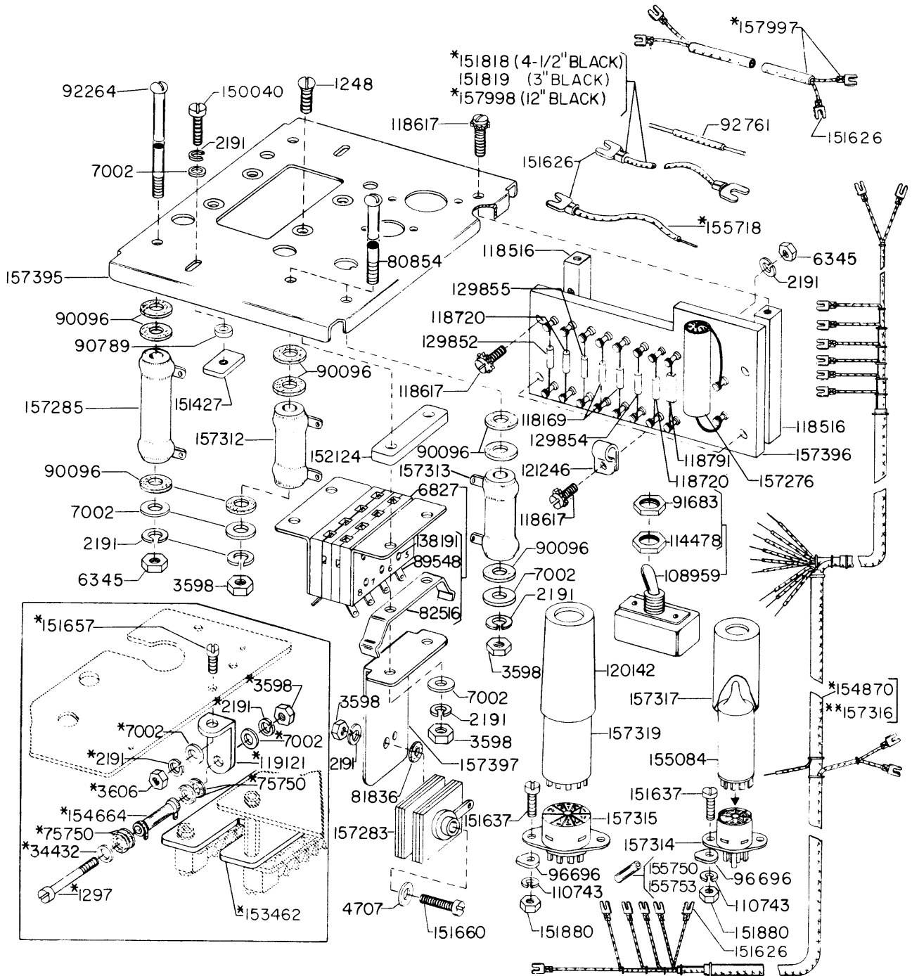
30RY LINE RELAY (SEE BULLETIN 1044B FOR COMPONENTS)
