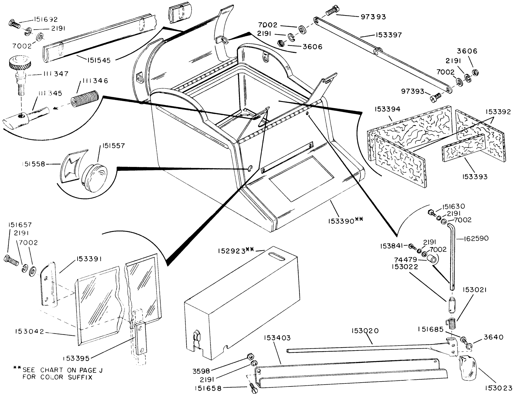
FIGURE 5-29 COVER ASSEMBLY
