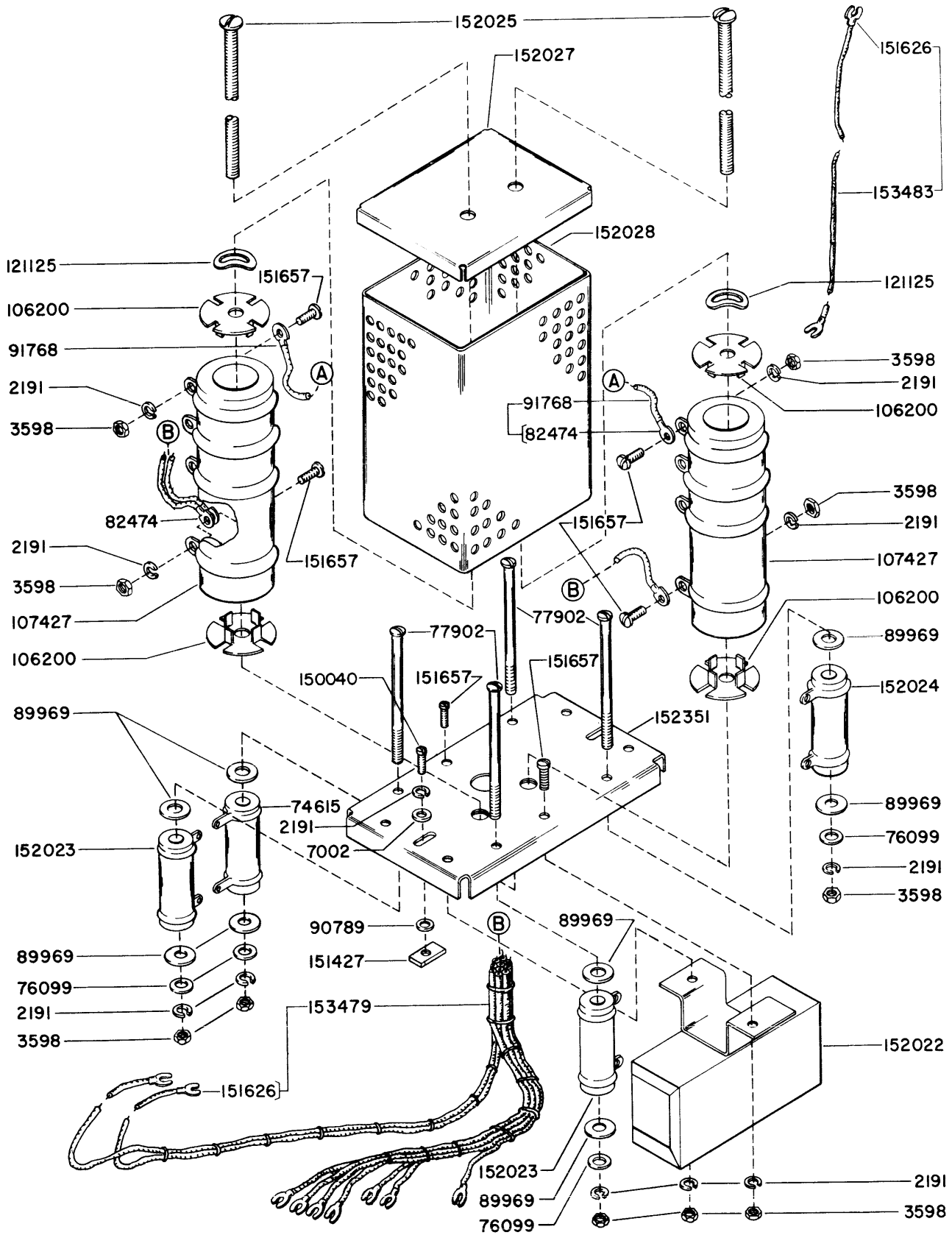
FIGURE 6-12. 152624 CAPACITOR-RESISTOR ASSEMBLY
