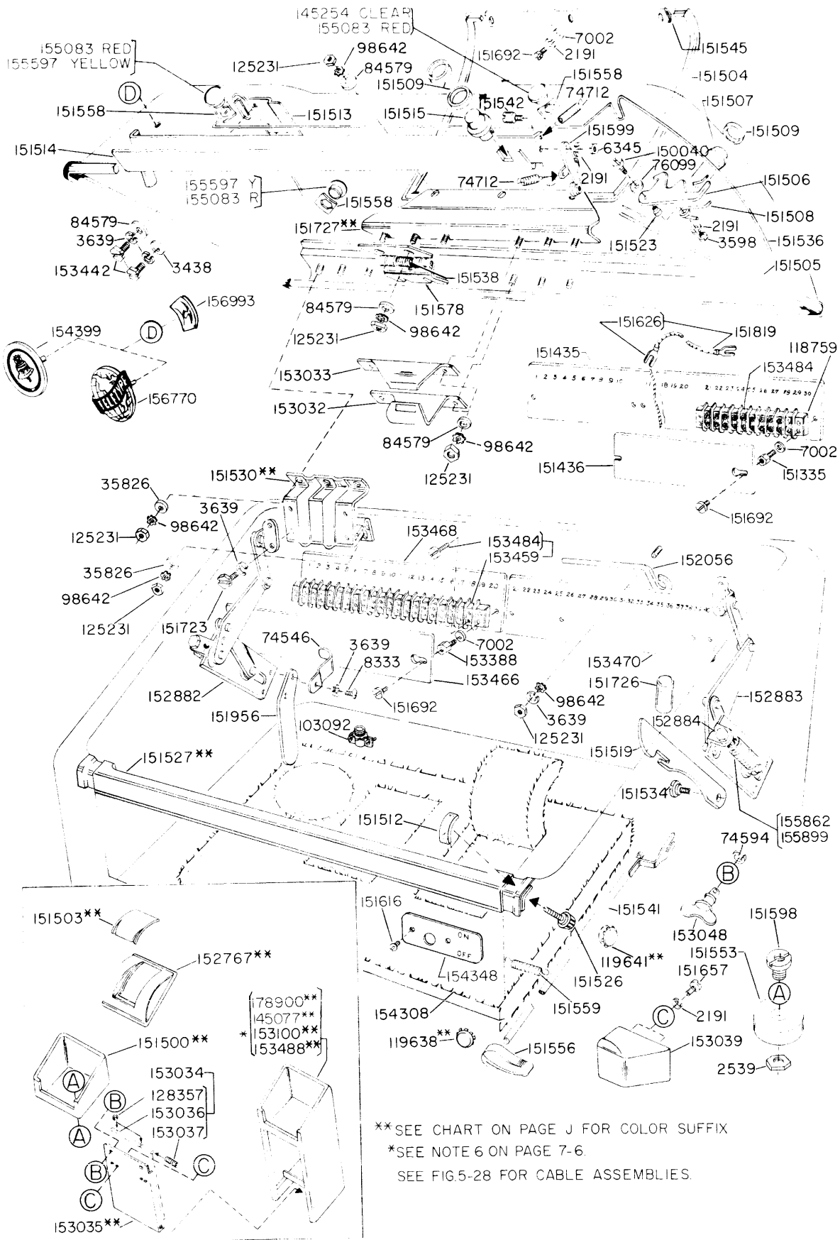
FIGURE 5-1. LAC202**,LAC203**,LAC204**,LAC213**,LAC215** AND LAC216** CABINETS
