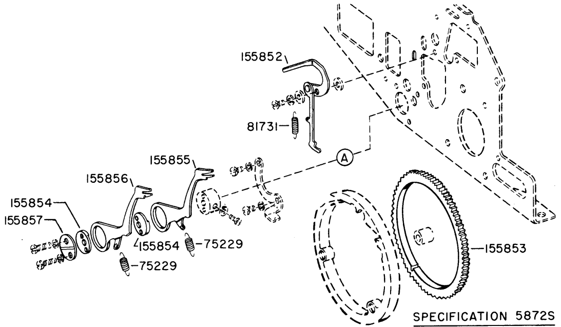
FIGURE 3-77. 154755 MODIFICATION KIT TO PROVIDE 5 SPACES PER INCH HORIZONTALLY
