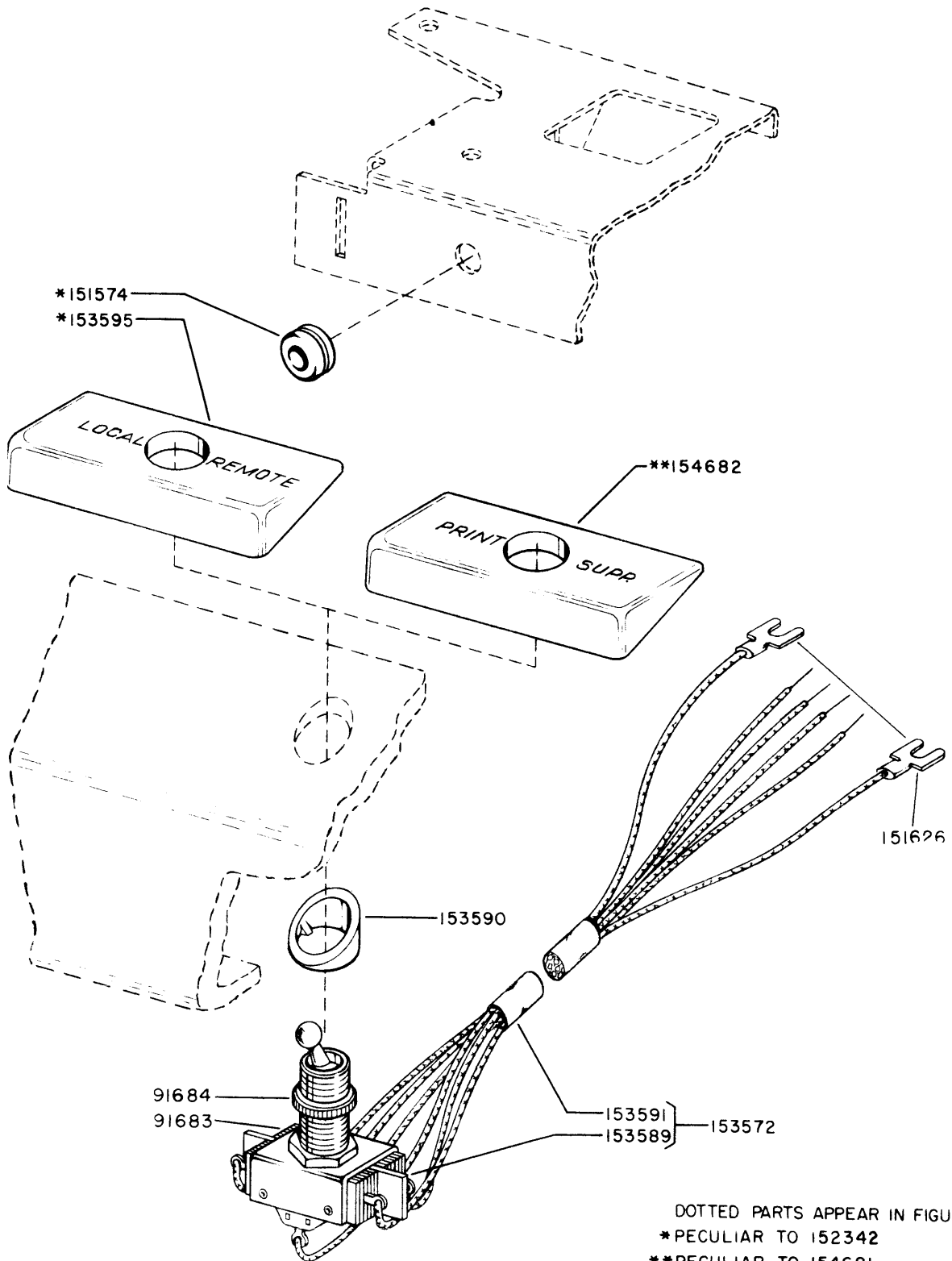
FIGURE I-22. 152342 MODIFICATION KIT TO PROVIDE LOCAL-REMOTE SWITCH (MARK II BASE)
