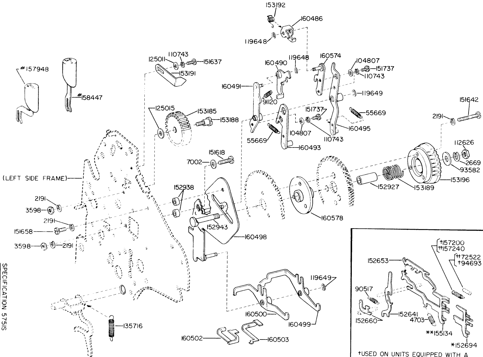
FIGURE 3-81 154770 MODIFICATION KIT TO PROVIDE VERTICAL TABULATION ON UPPER CASE "J" AND "Z"
