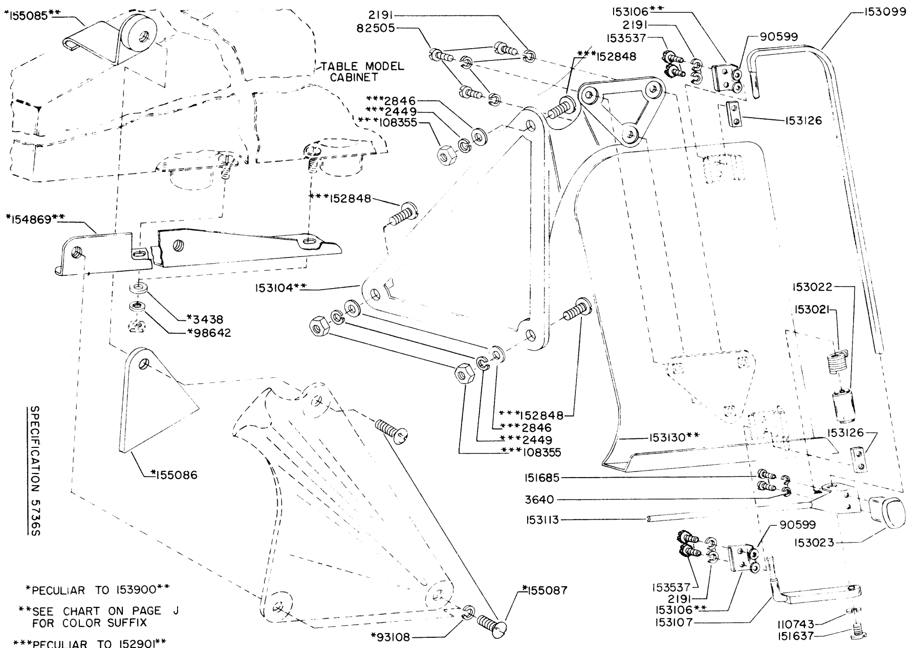
FIGURE 5-10. 152901** AND 153900** MODIFICATION KITS TO PROVIDE OFFSET COPYHOLDERS
