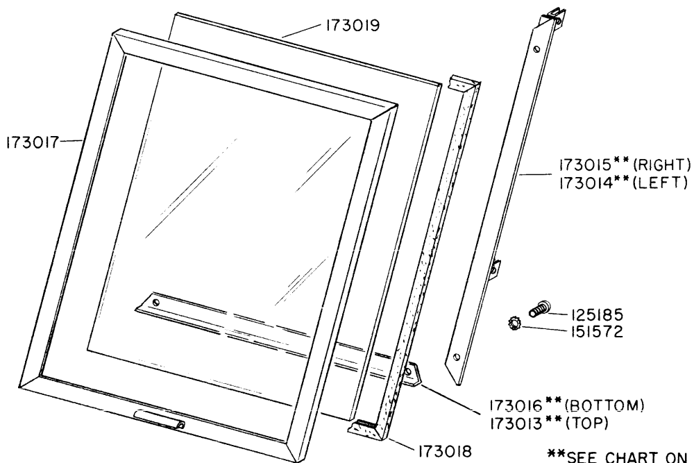
FIGURE 5-43. 172700** DOOR ASSEMBLY
