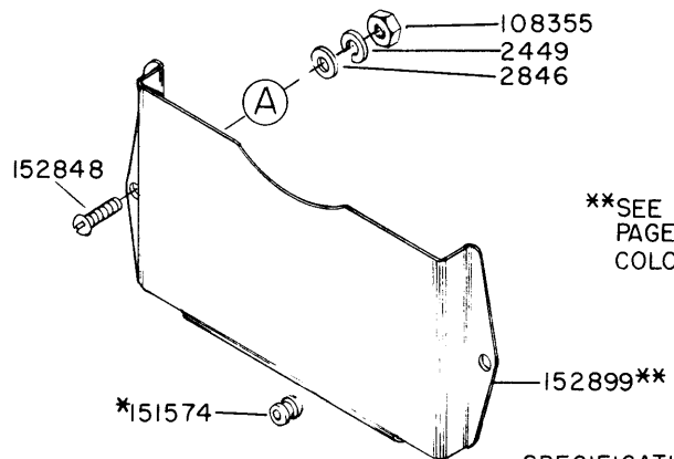
FIGURE 5-8. 152910** MODIFICATION KIT TO PROVIDE DIRECTORY HOLDER
