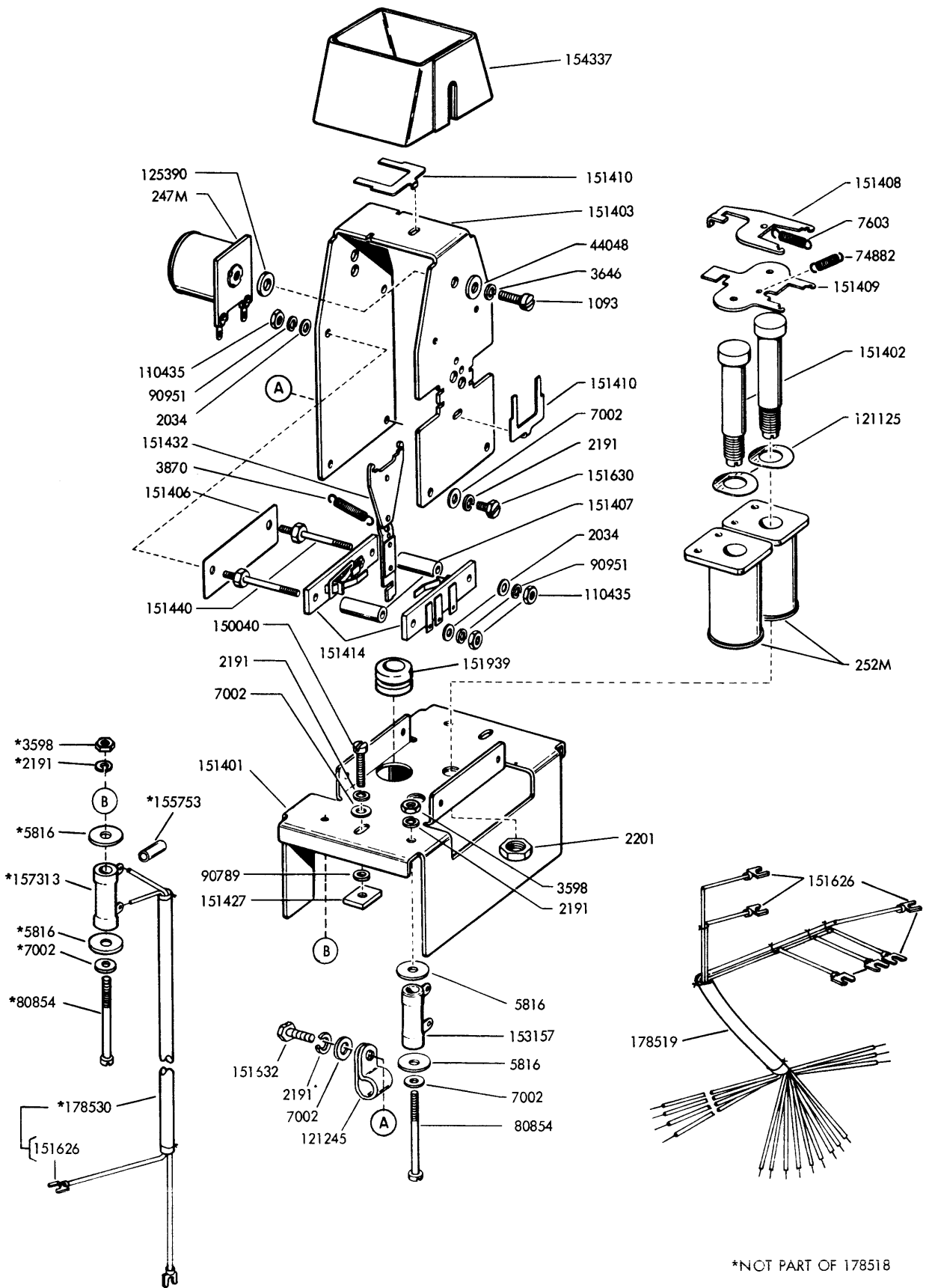
FIGURE 7A-13. 178518 MOTOR CONTROL ASSEMBLY
