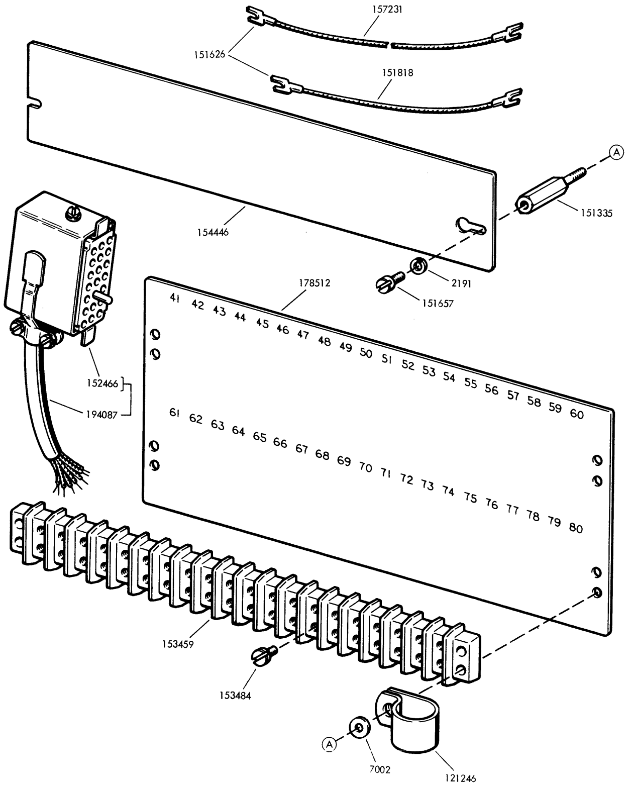
FIGURE 7A-11. 194086 MODIFICATION KIT TO ADAPT WALL MOUNTED PRINTER FOR SELECTIVE CALLING
