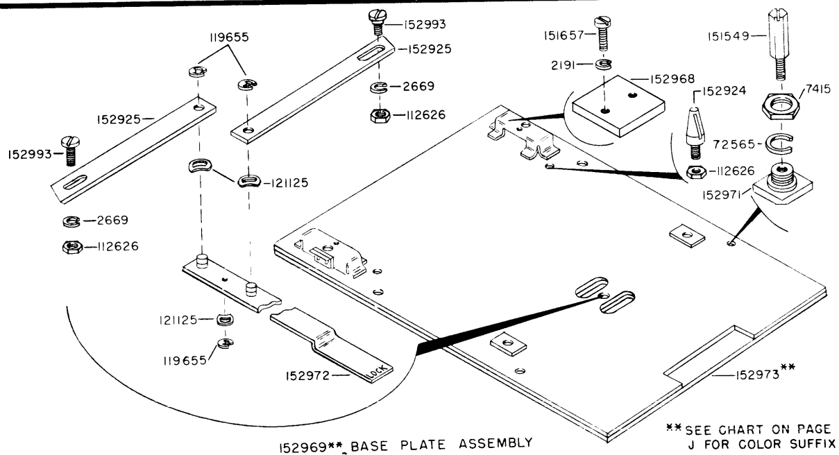
FIGURE 5-30. VARIABLE FEATURES FOR LPC202** AND LPC203** COVERS
