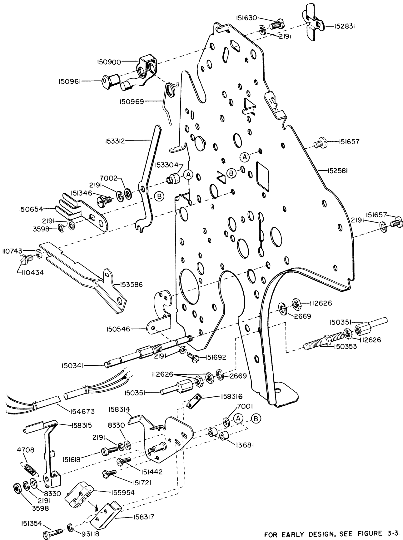
FIGURE 3-1 LEFT SIDE FRAME MECHANISM
