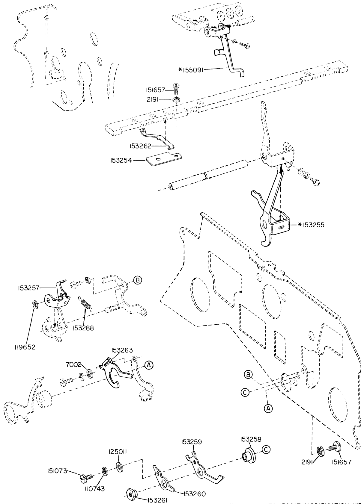
FIGURE 3-88. 152917 AND 157510 MODIFICATION KITS TO PROVIDE LOCAL BACK SPACE
