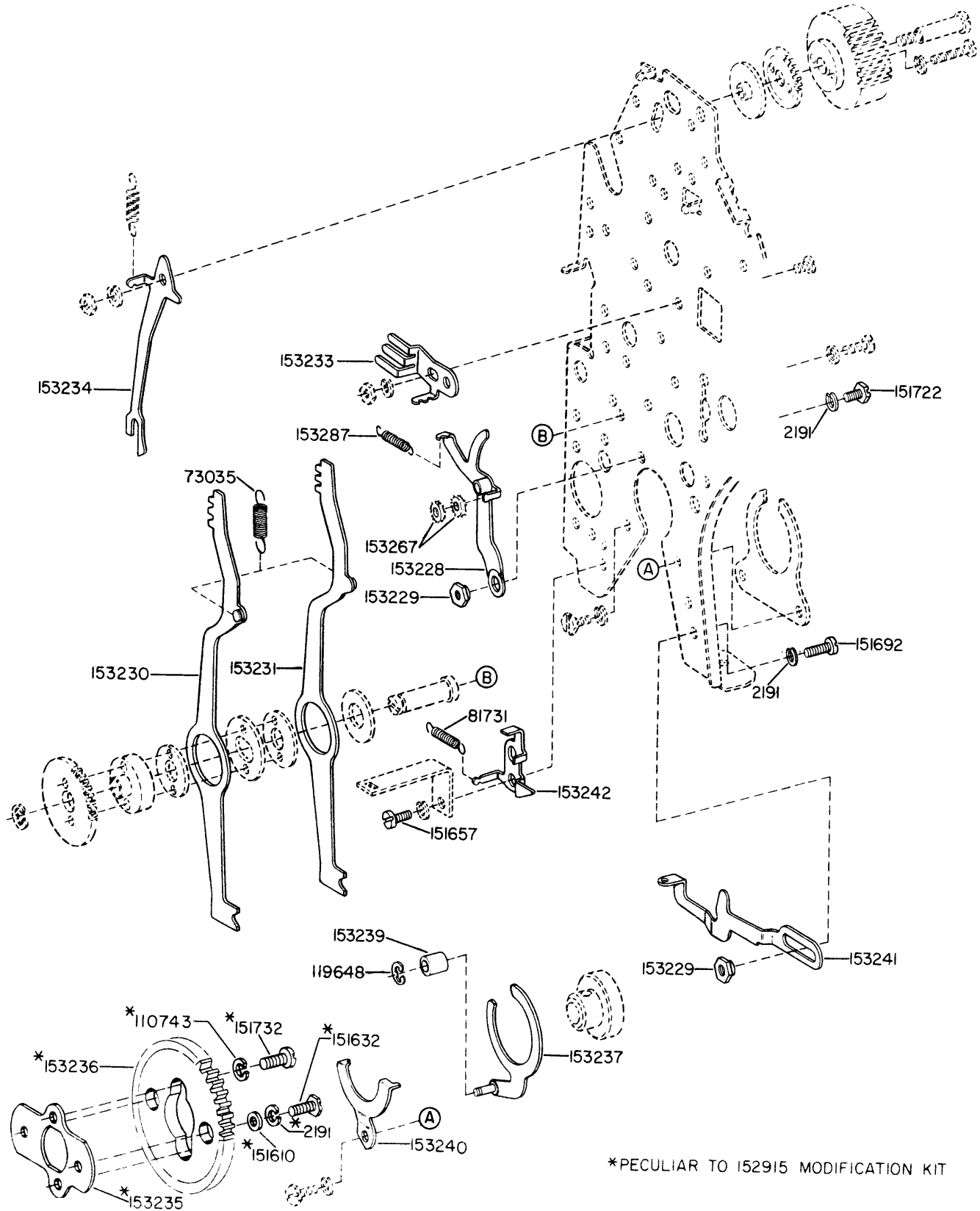
FIGURE 3-68 152915 AND 157511 MODIFICATION KITS TO PROVIDE LOCAL REVERSE LINE FEED
