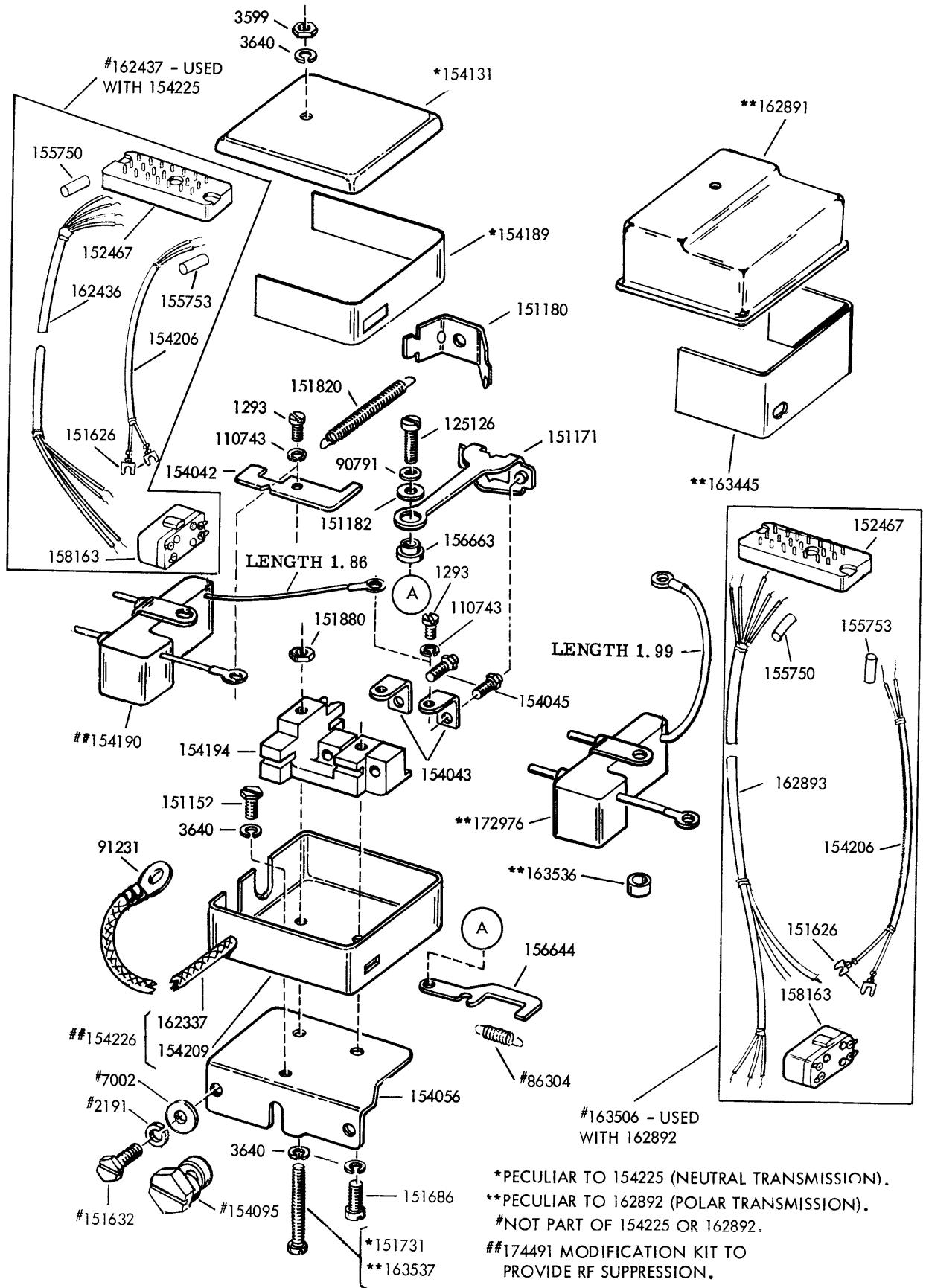
FIGURE 2-14. 154225 AND 162892 CONTACT BOX ASSEMBLIES WITH RF SUPPRESSION - NEUTRAL AND POLAR TRANSMISSION
