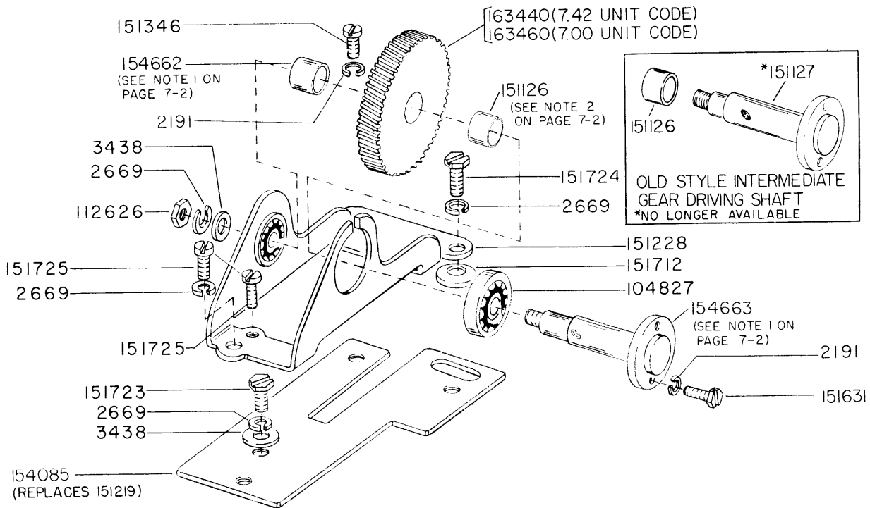
FIGURE I-6 INTERMEDIATE GEAR MECHANISM
