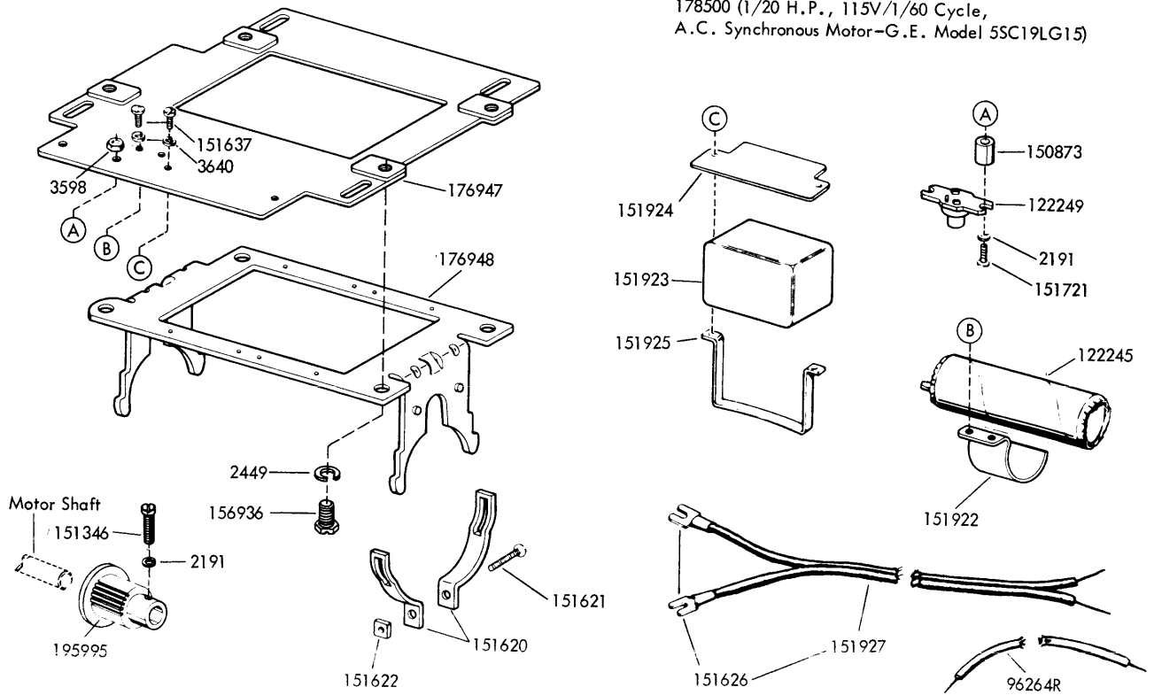
FIGURE 7A-5. LMU27 SYNCHRONOUS MOTOR UNIT
