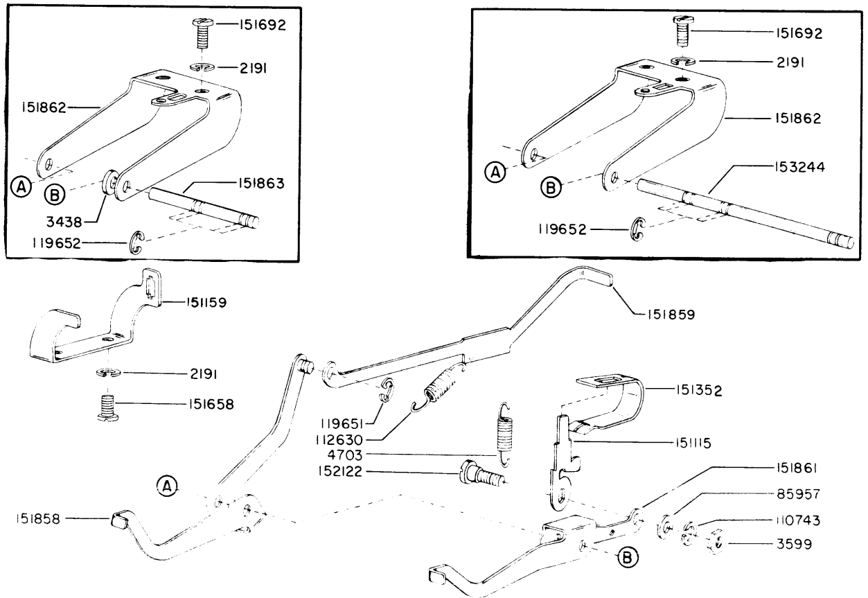
FIGURE I-8. KEYBOARD LOCK AND LOCAL LINE FEED MECHANISM
