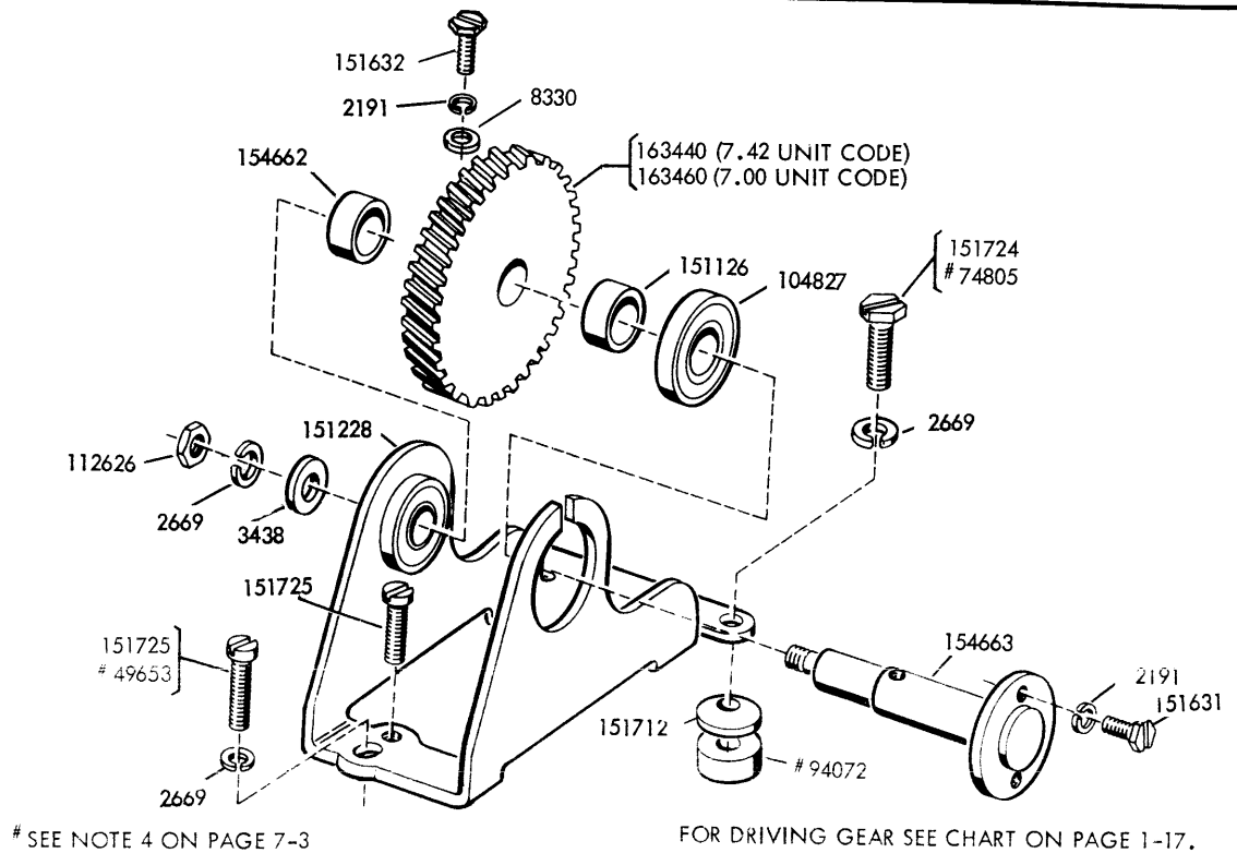
FIGURE 2-3 INTERMEDIATE GEAR MECHANISM
