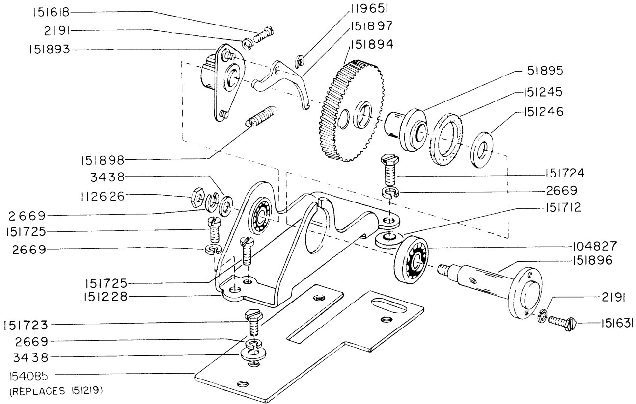
FIGURE I-5 INTERMEDIATE GEAR MECHANISM
