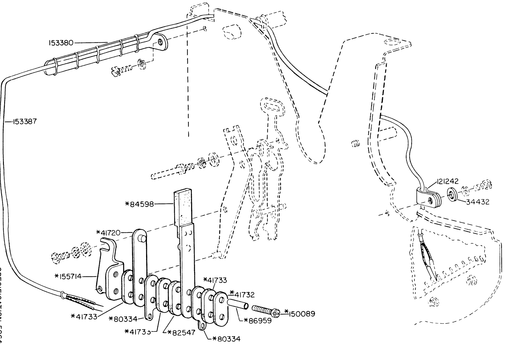
FIGURE 3-84. 154780 MODIFICATION KIT TO PROVIDE HORIZONTAL TABULATOR XD CONTROL
