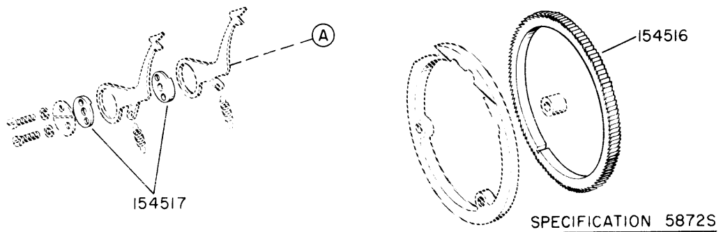
FIGURE 3-79. 154792 MODIFICATION KIT TO PROVIDE 12 SPACES PER INCH HORIZONTALLY
