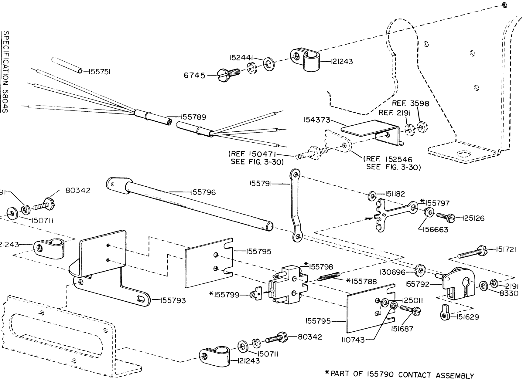
FIGURE 3-85. 154785 MODIFICATION KIT TO PROVIDE UNIVERSAL CONTACTS CHANGE II
