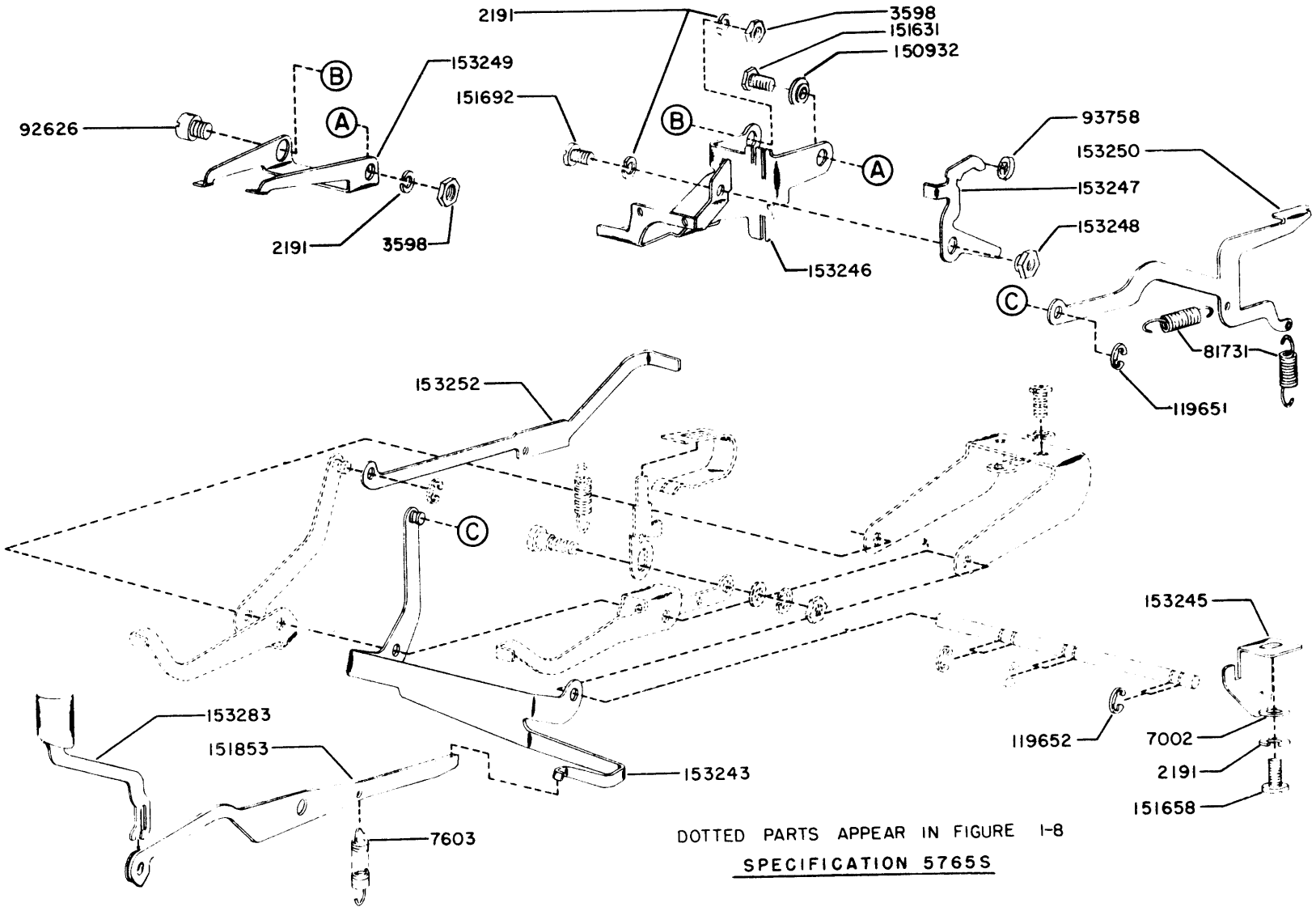
FIGURE 1-25. 152916 MODIFICATION KIT TO PROVIDE LOCAL REVERSE LINE FEED MECHANISM (MARK II KEYBOARD)
