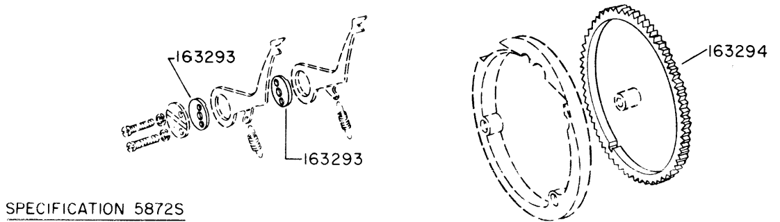
FIGURE 3-90 163292 MODIFICATION KIT TO PROVIDE 8 SPACES PER INCH MECHANISM
