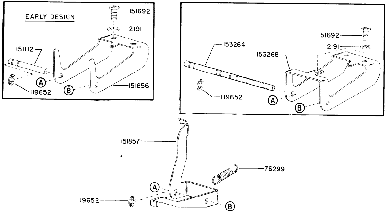
FIGURE I-7. CARRIAGE RETURN MECHANISM
