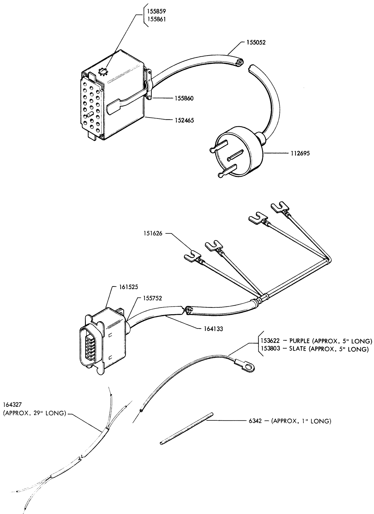
FIGURE 1-26. AUXILIARY CABLES (MARK II KEYBOARD OR BASE)
