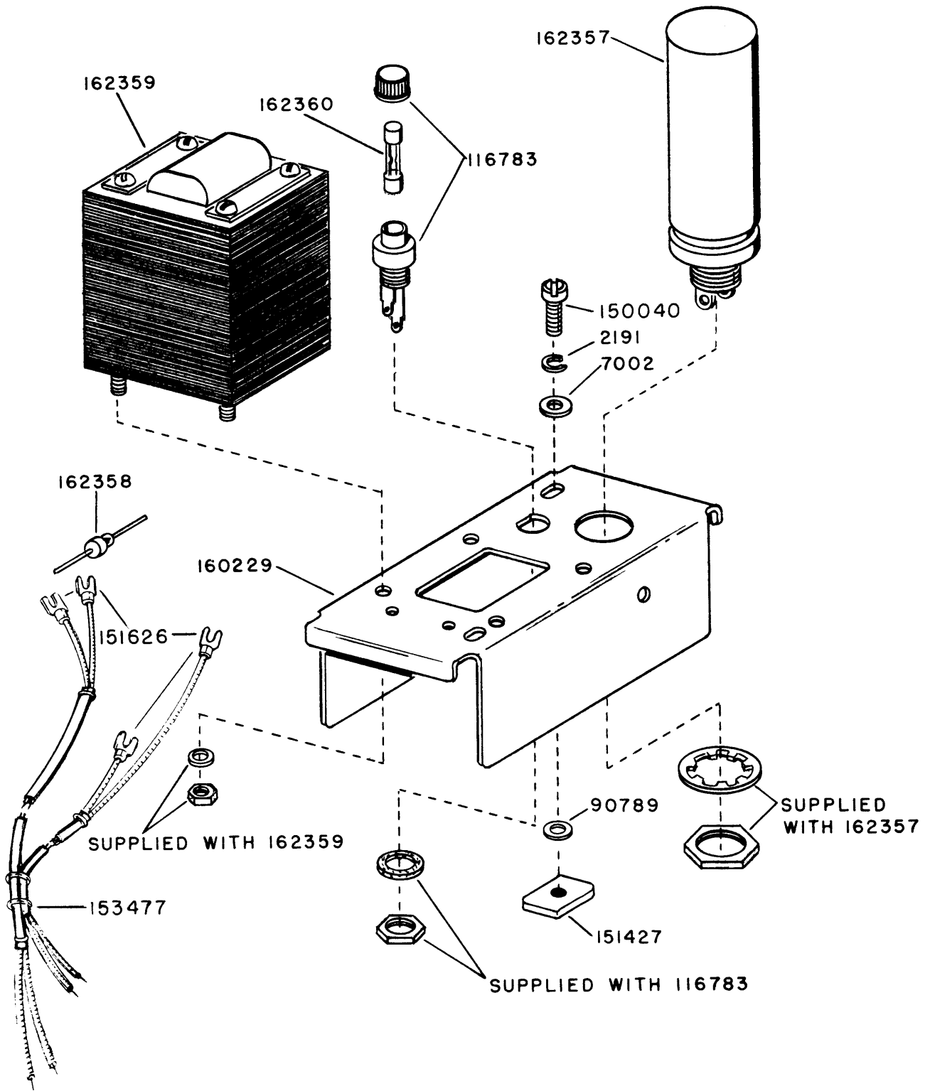
FIGURE 6-25. 162361 RECTIFIER AND CABLE ASSEMBLY (500MA)
