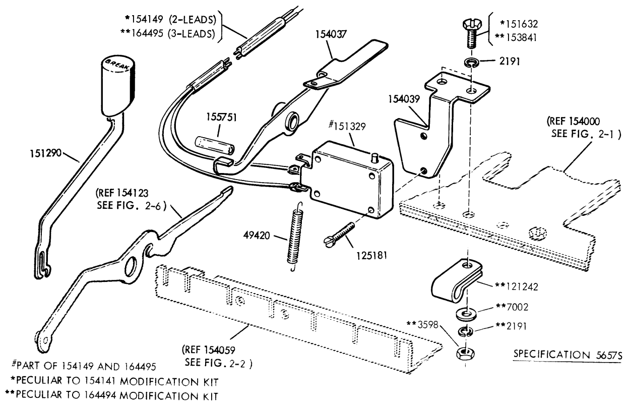
FIGURE 2-17. 154141 AND 164494 MODIFICATION KIT TO PROVIDE ELECTRICAL SIGNAL LINE BREAK MECHANISM (MARK III KEYBOARD)
