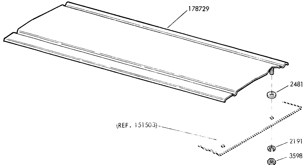
FIGURE 5-60. 174458 MODIFICATION KIT TO PROVIDE LAC CABINET WITH A PAPER TEARING PLATE
