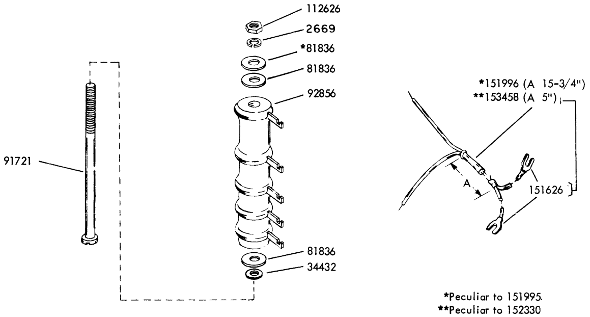
FIGURE 6-4. 151995 AND 152330 MODIFICATION KITS TO ADD LINE PAD RESISTOR TO LESU
