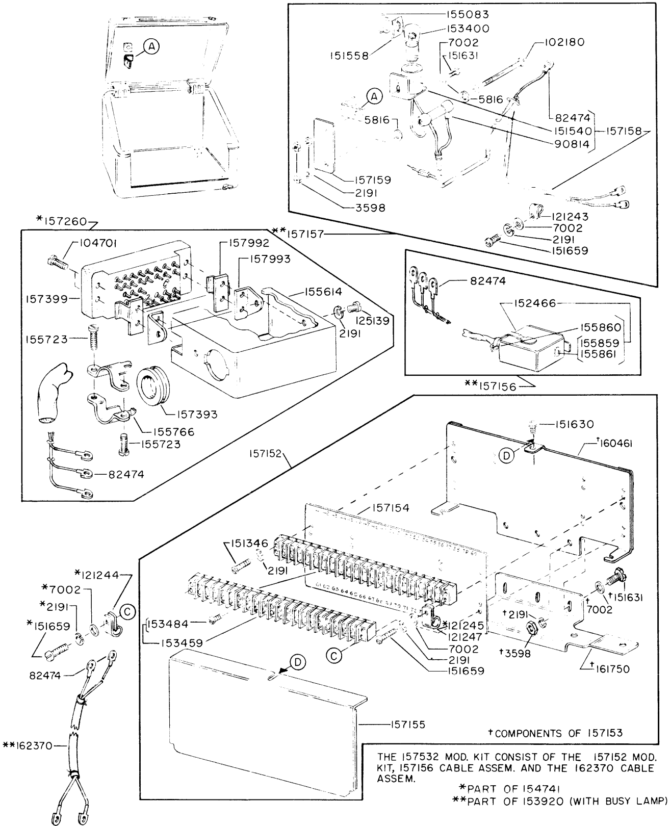
FIGURE 5-12. 153920 AND 154741 MODIFICATION KITS TO ADAPT A CABINET FOR SELECTIVE CALLING
