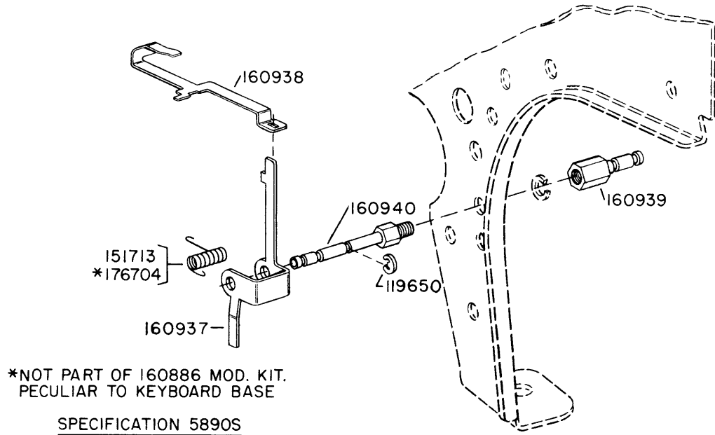
FIGURE 3-89. 160886 MODIFICATION KIT TO PROVIDE LOCAL FORM FEED-OUT (RECEIVING ONLY BASE)
