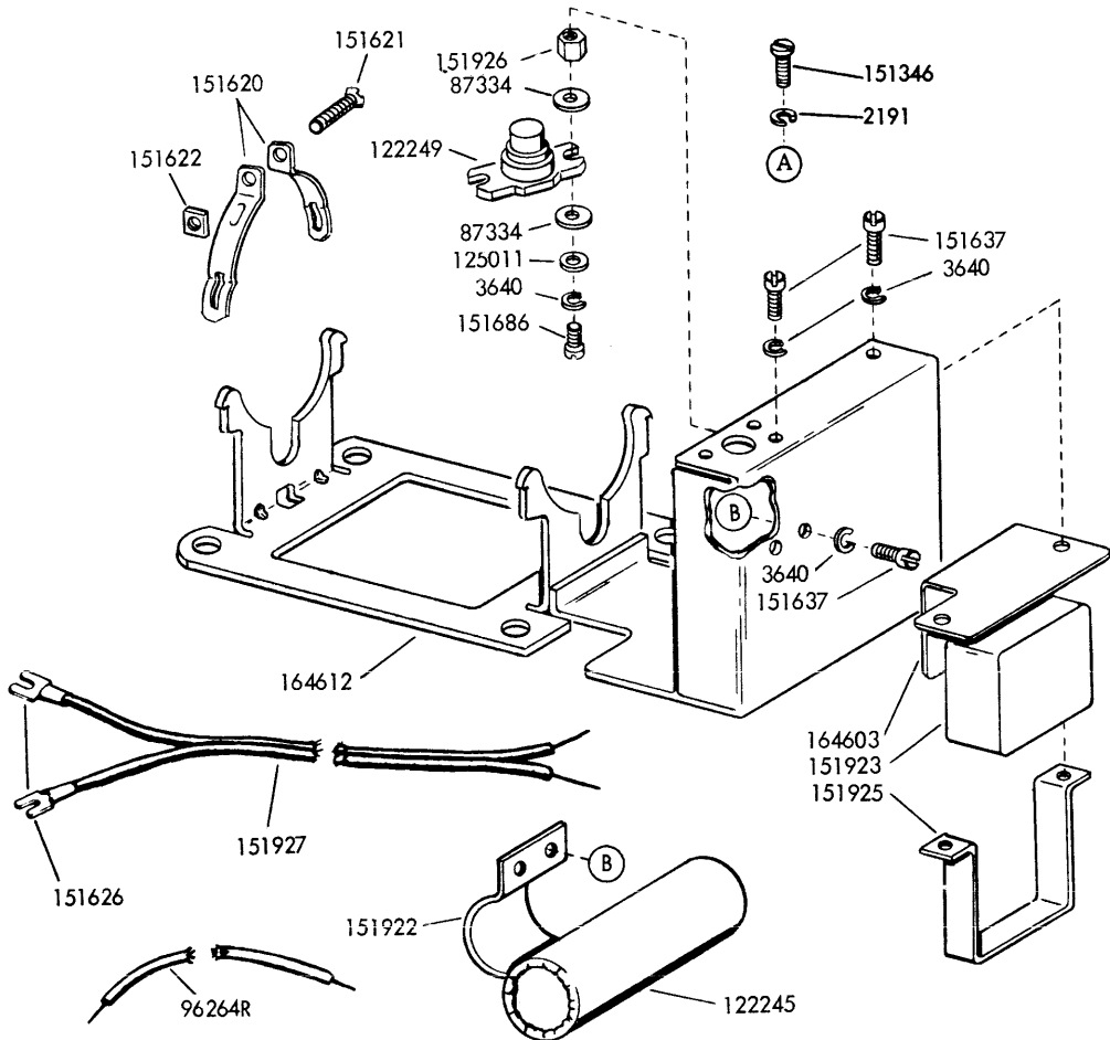
FIGURE 4-7. LMU21 SYNCHRONOUS MOTOR UNIT
