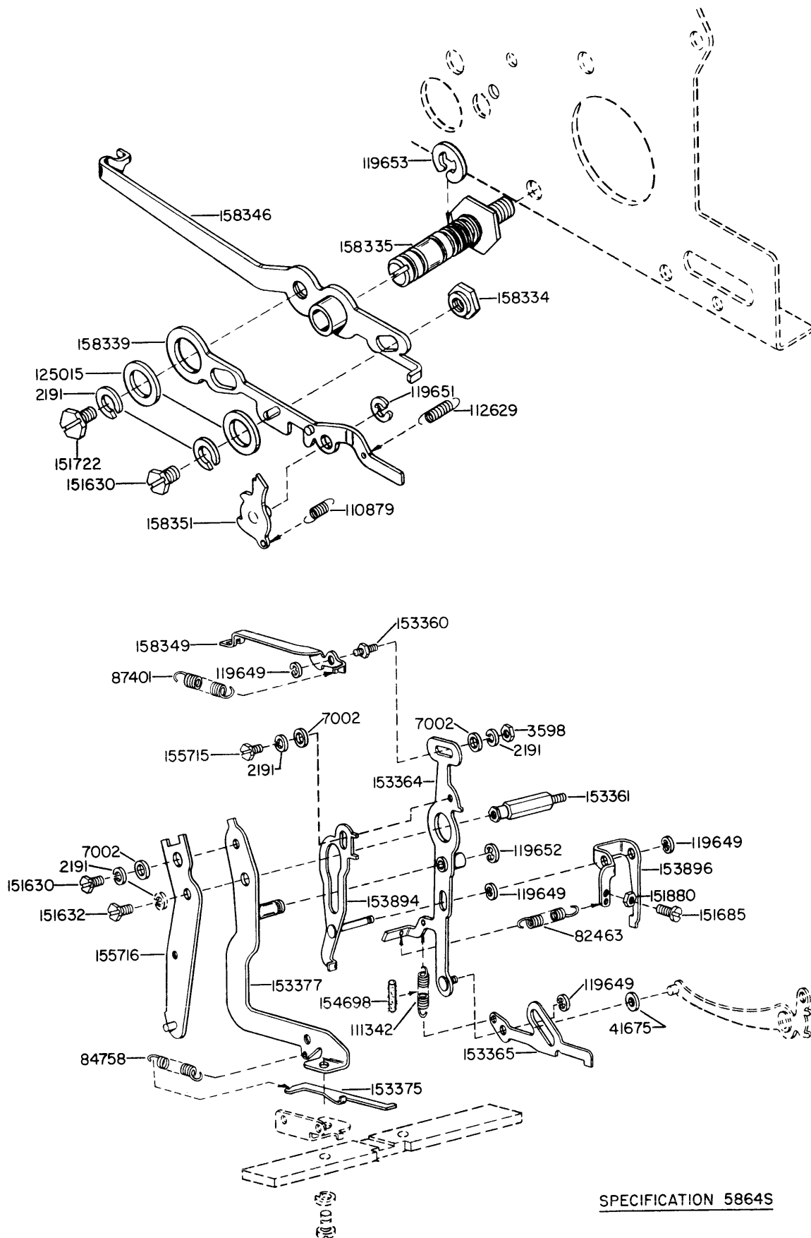
FIGURE 3-86. 157508 MODIFICATION KIT TO PROVIDE HORIZONTAL TABULATION (CONTINUED ON NEXT PAGE)
