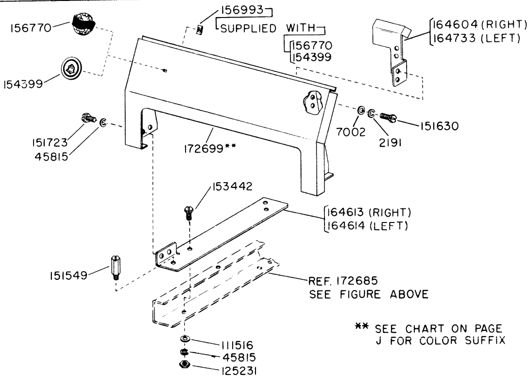
FIGURE 5-38. SLIDE MECHANISM (LBAC211**)
