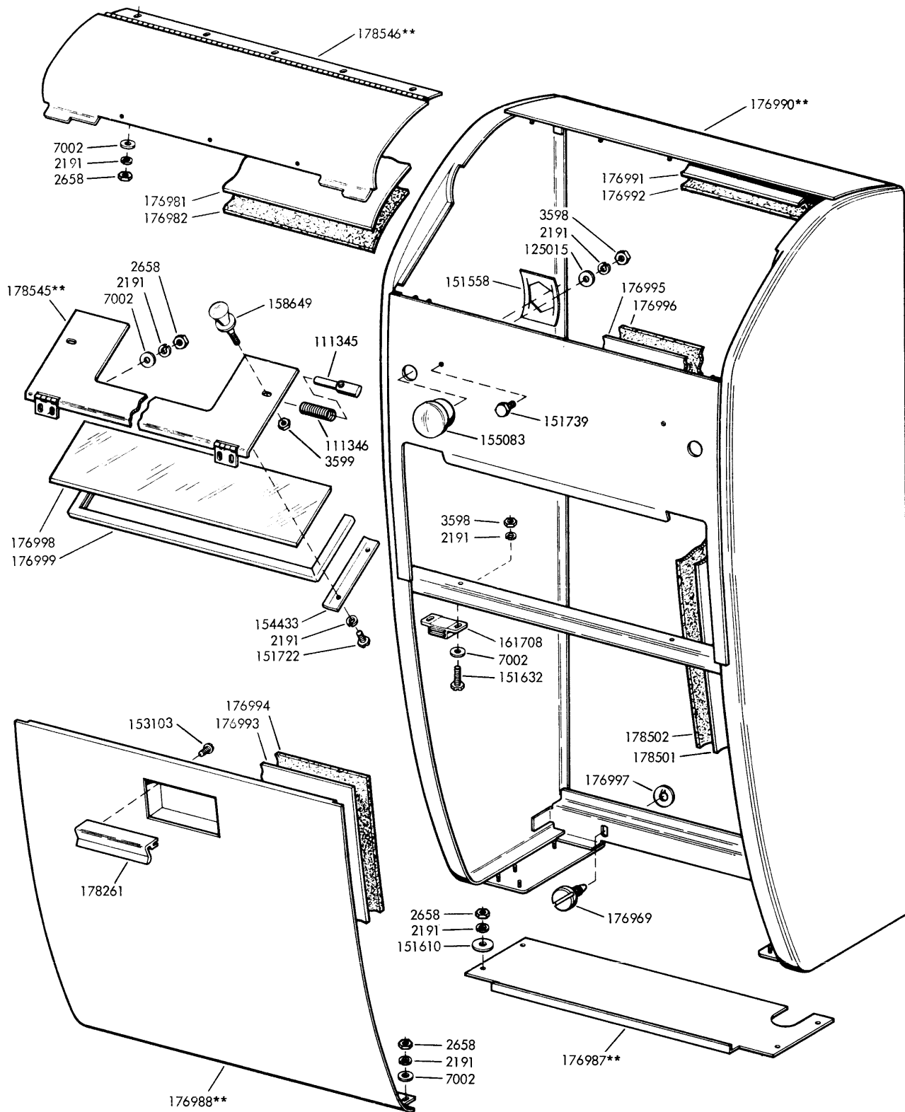
FIGURE 7A-16. WALL MOUNTED CABINET
