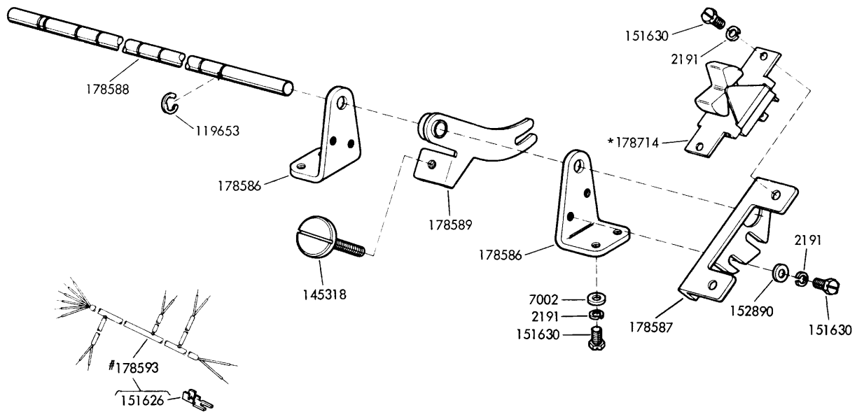
FIGURE 7A-3. TRIP LEVER MECHANISM
