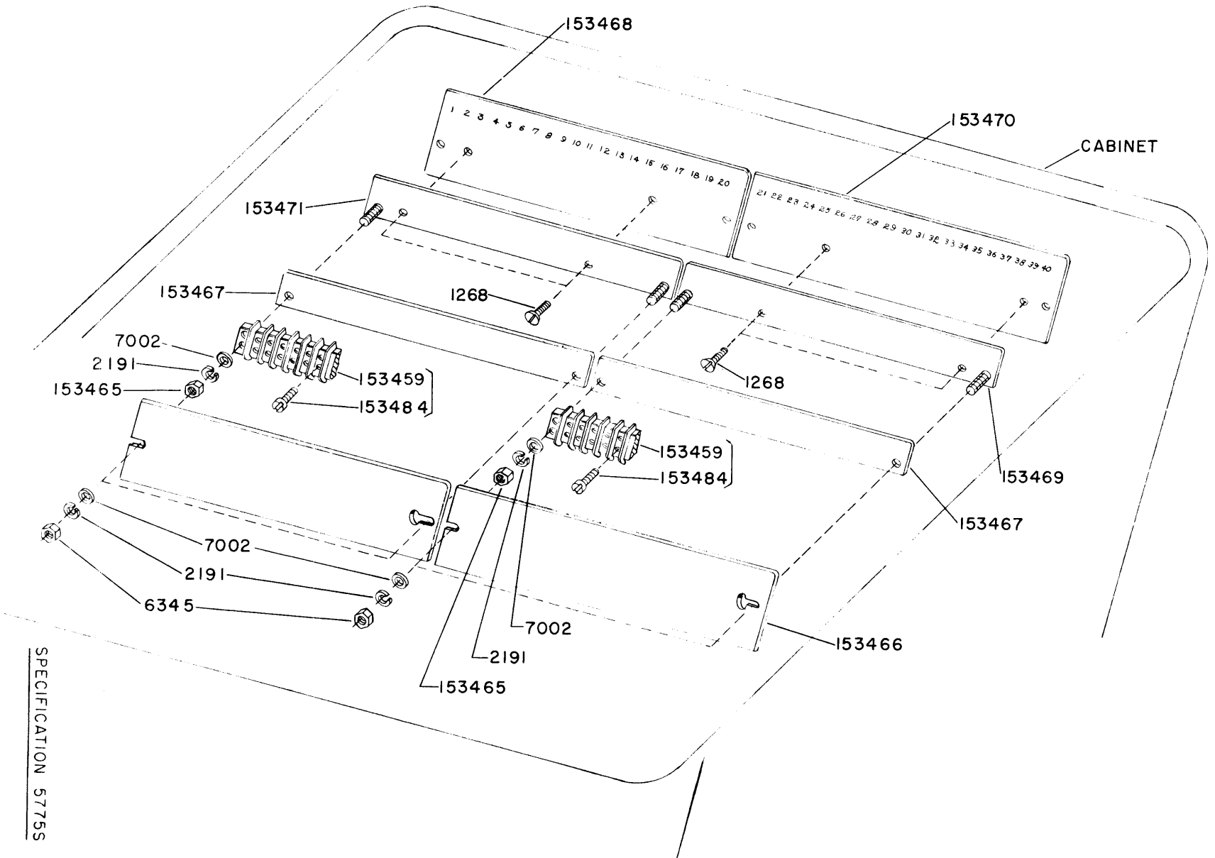
FIGURE 5-13. 152319 MODIFICATION KIT TO PROVIDE ADDITIONAL TERMINAL CONNECTIONS ON CABINET
