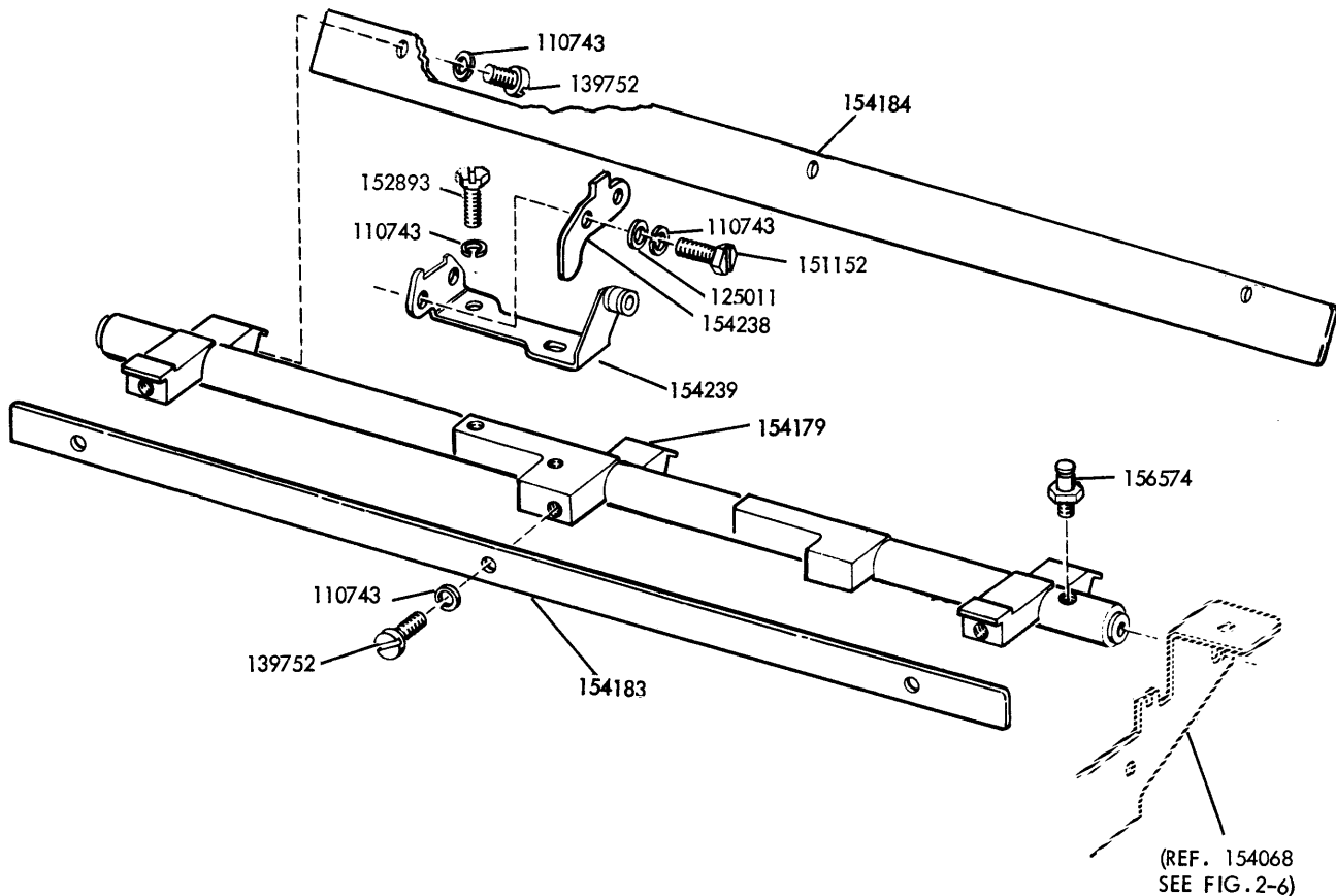
FIGURE 2-7. UNIVERSAL BAIL MECHANISM
