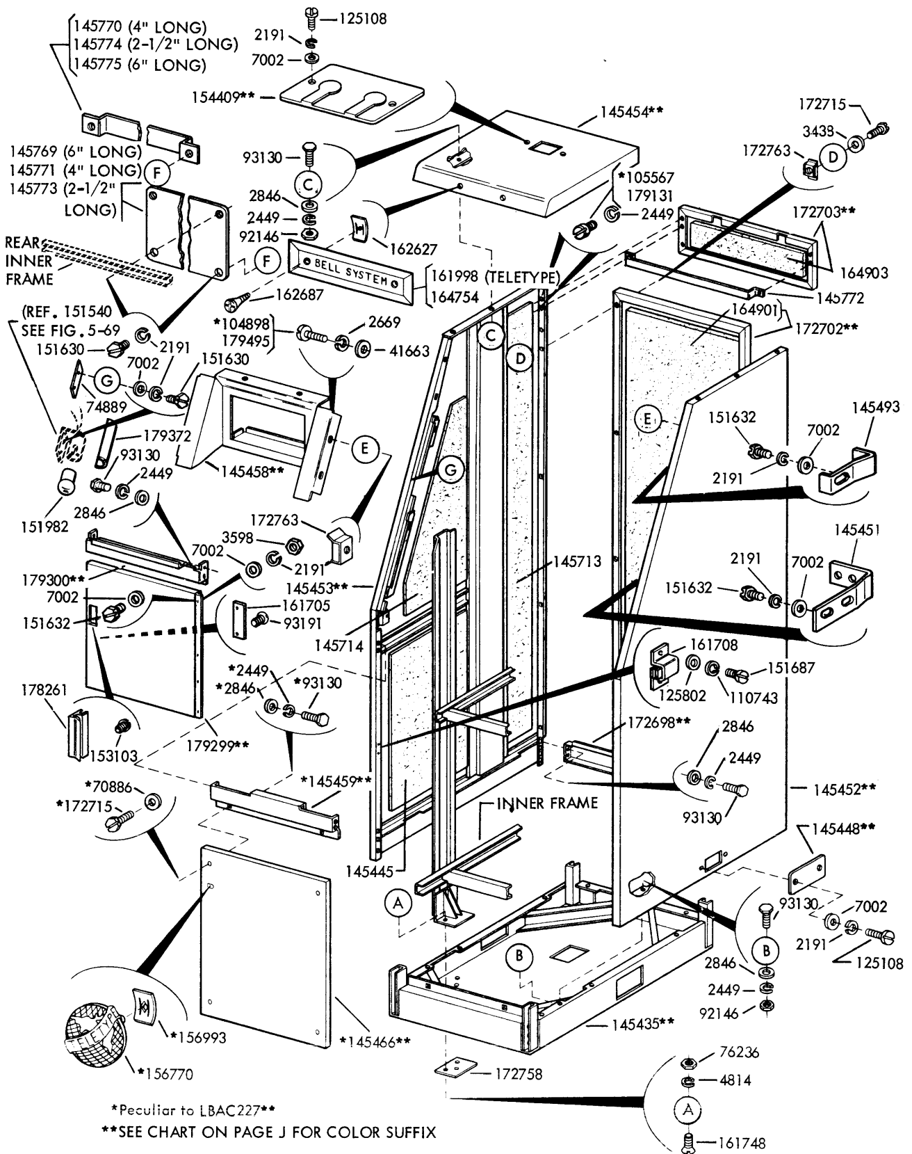
FIGURE 5-46. CABINET BODY ASSEMBLY (LBAC227** AND LBAC233**)
