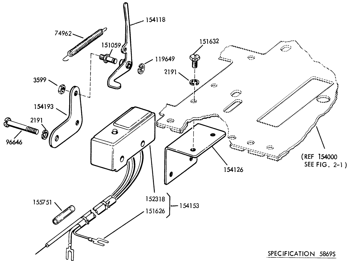
FIGURE 2-16. 154147 MODIFICATION KIT TO PROVIDE LOCAL PAPER FEED-OUT MOTOR STARTING MECHANISM (MARK III KEYBOARD)
