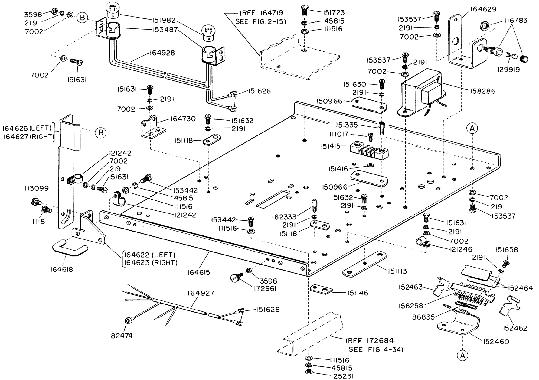
FIGURE 5-44. RECEIVING ONLY BASE PLATE (LBAC211**)
