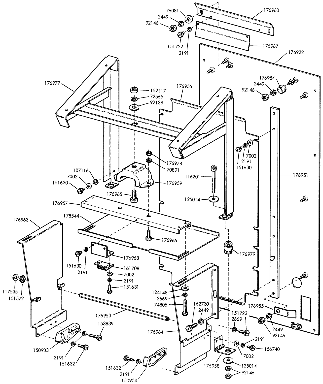
FIGURE 7A-15. BACK PLATE ASSEMBLY
