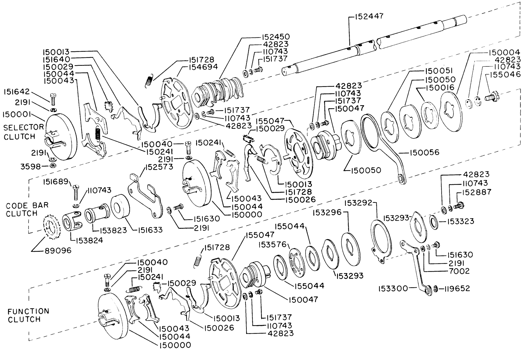
FIGURE 3-19. MAIN SHAFT MECHANISM
