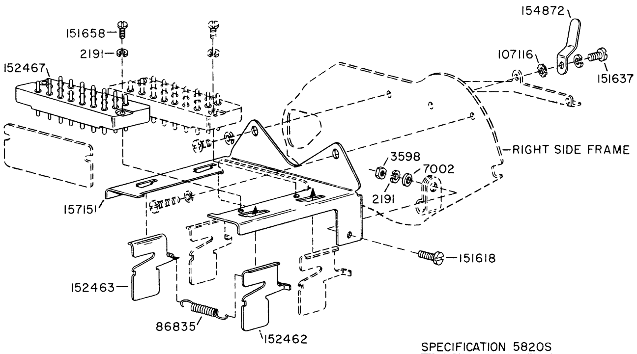
FIGURE 3-67. 153919 MODIFICATION KIT TO PROVIDE AUXILIARY CONNECTOR
