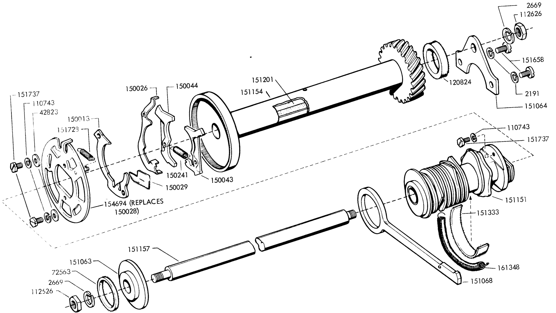
FIGURE 1-12. SIGNAL GENERATOR MECHANISM
