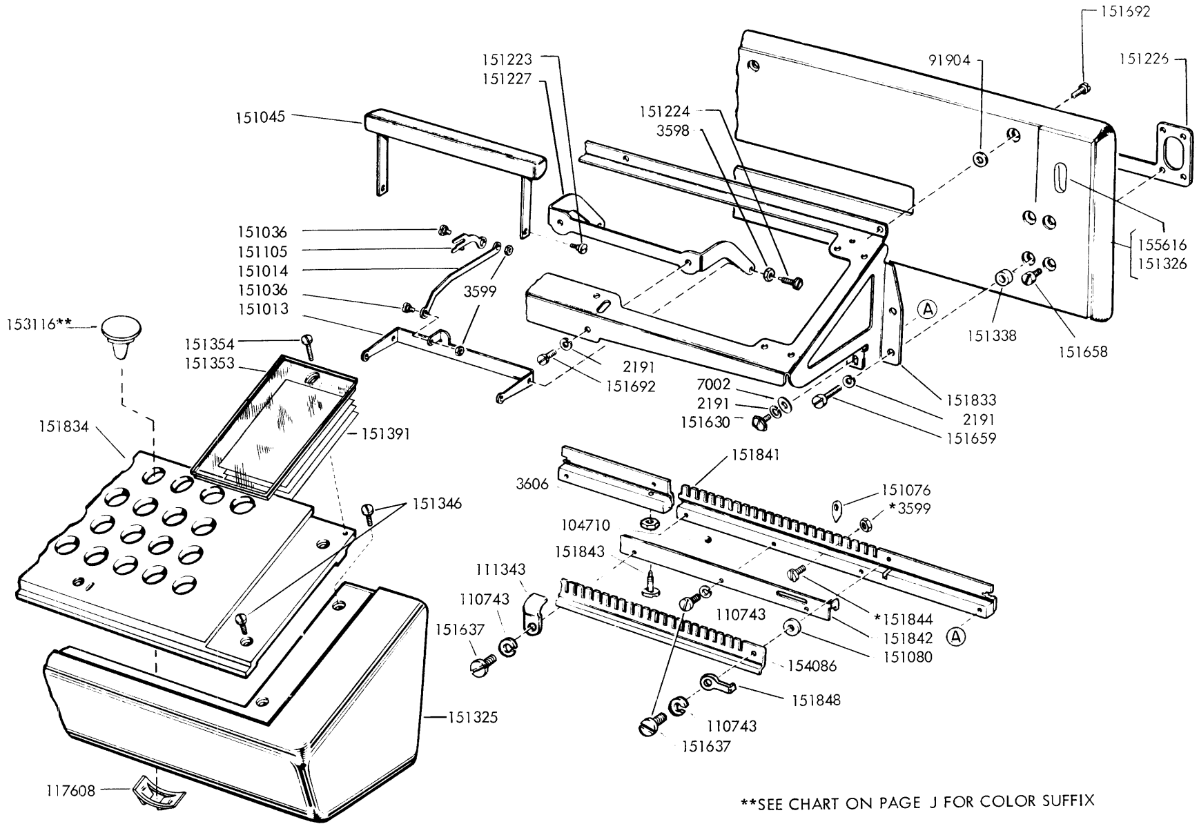
FIGURE 1-9. KEYBOARD MECHANISM
