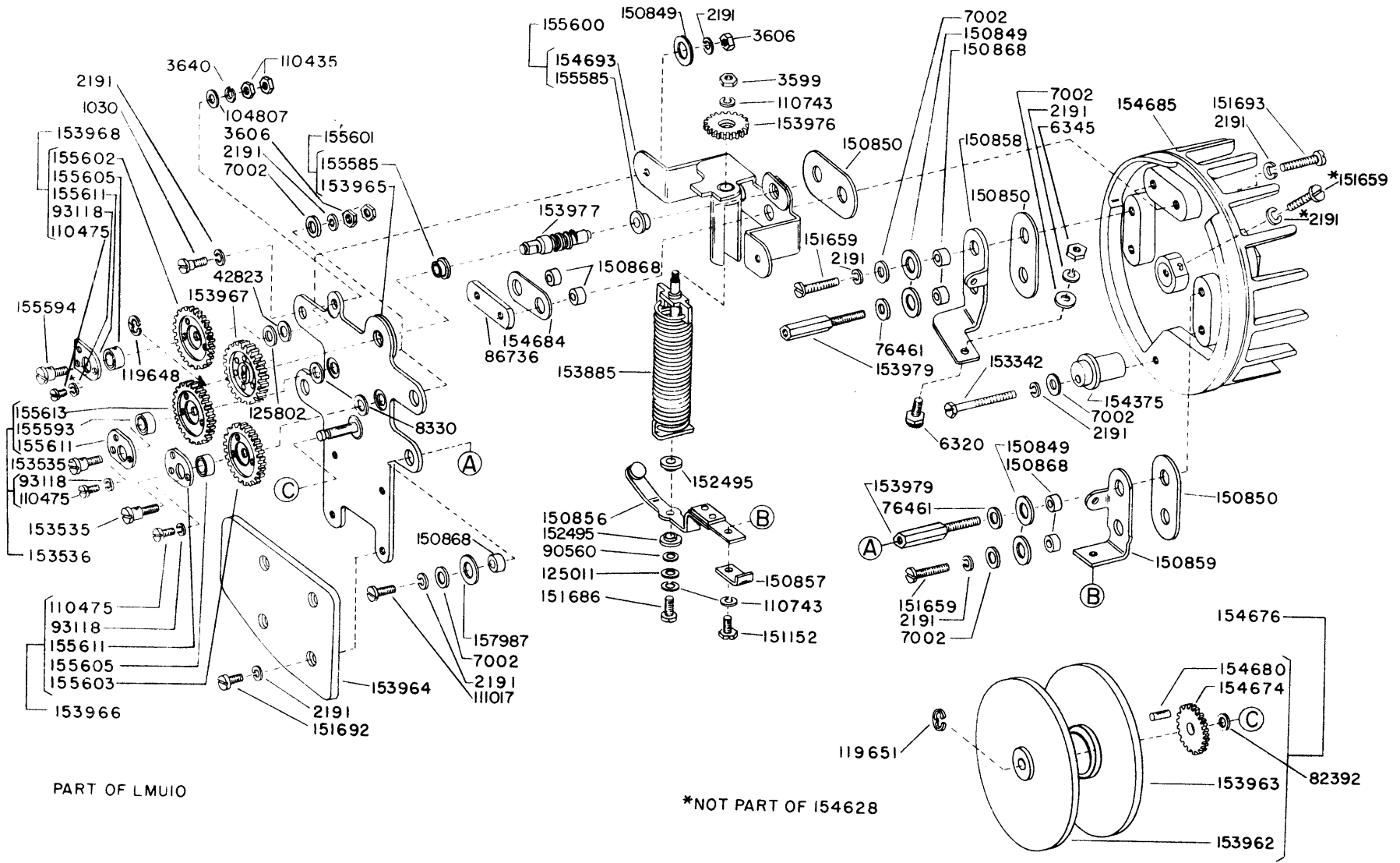
FIGURE 4-6. 154628 GOVERNOR ASSEMBLY
