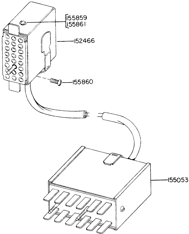
FIGURE 3-75. I55051 AUXILIARY CABLE ASSEMBLY
