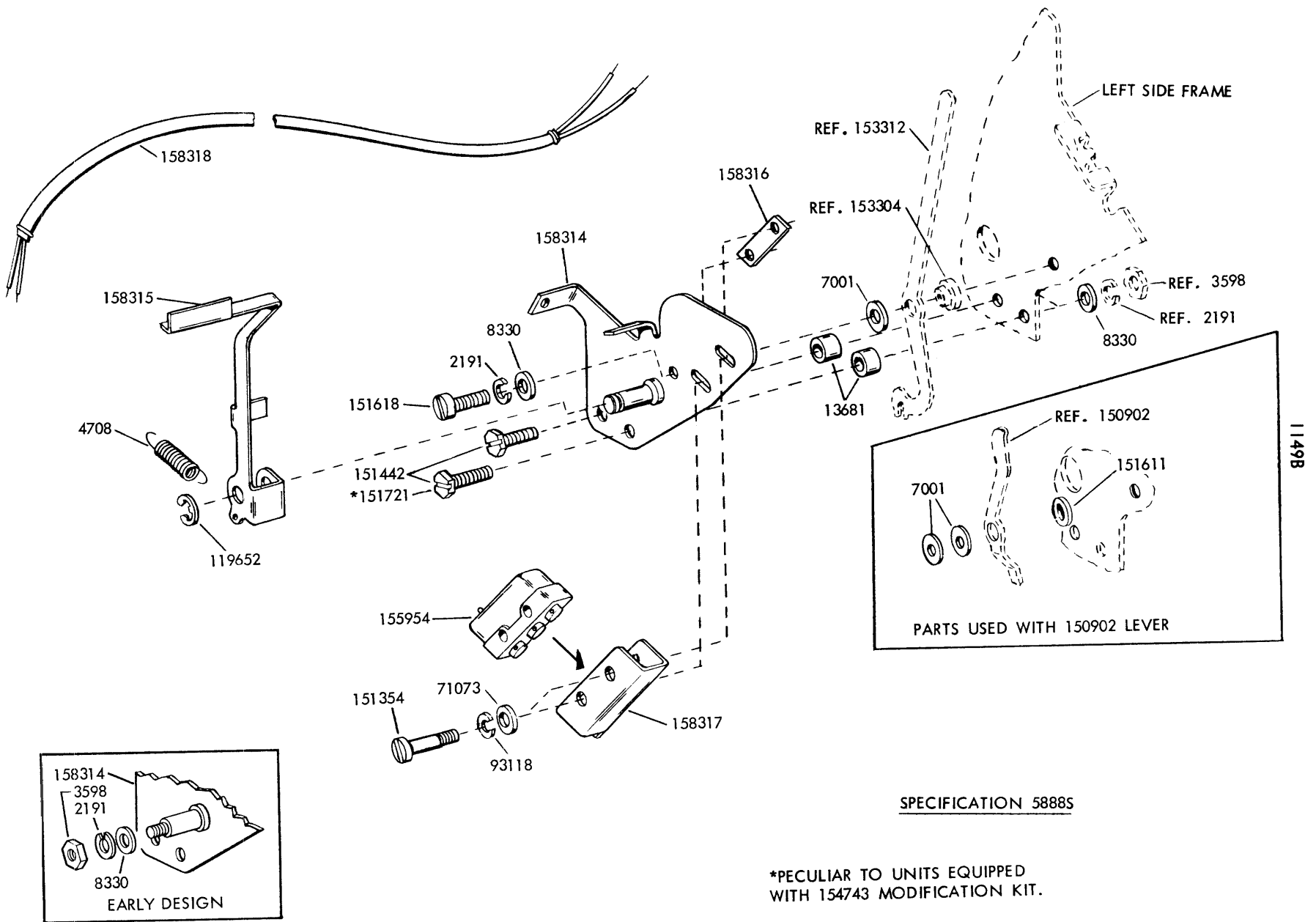
FIGURE 3-99. 159366 MODIFICATION KIT TO EQUIP A FRICTION FEED PRINTER WITH PAPER-OUT ALARM CHANGE II
