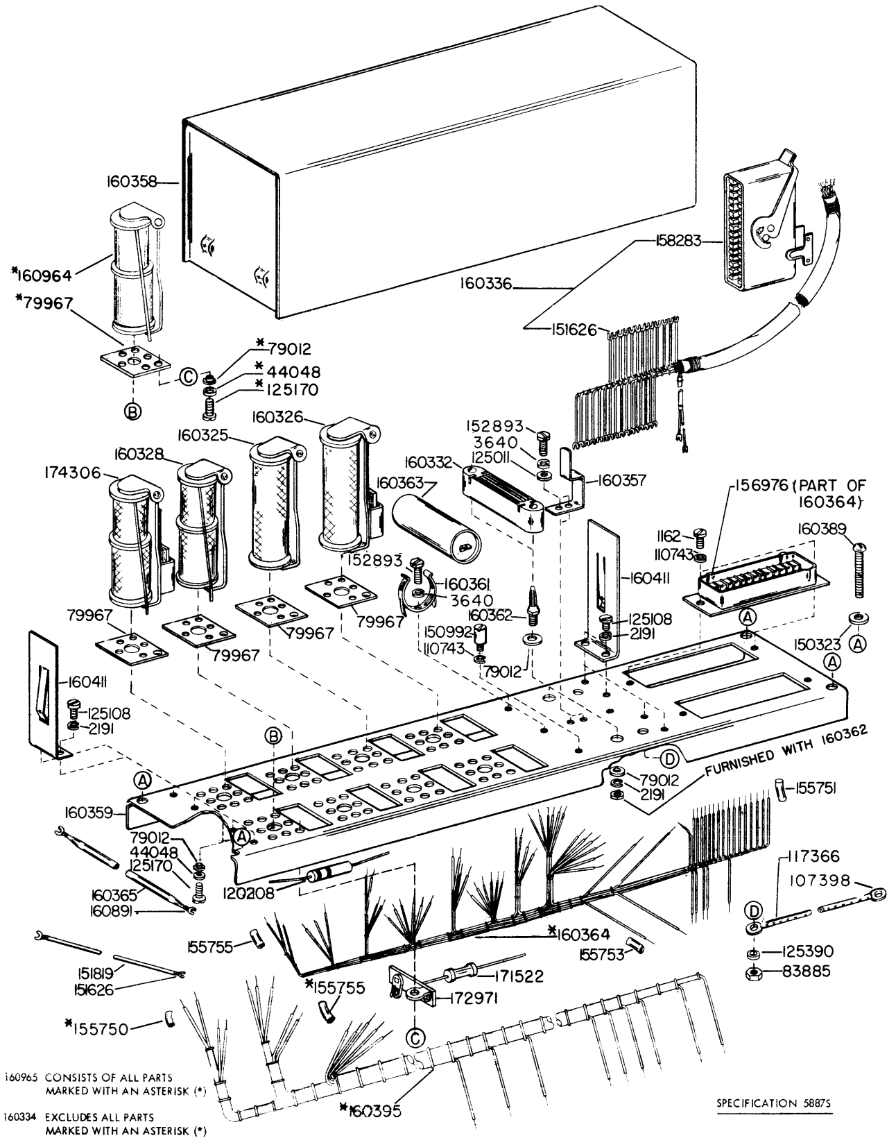
FIGURE 6-22. 160966 MODIFICATION KIT TO PROVIDE TRANSMITTER AND REPERFORATOR CONTROL
